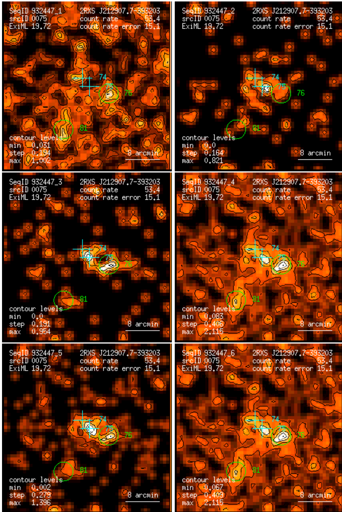
Figure 75: RASS 932447: detection 0075: band rate images, Gaussian filter: (1) PSPC channels 11 – 41, (2) 52 – 90, (3) 91 – 201, (4) 11 – 235, (5) 52 – 201, (6) 11 – 201. Broad band rates in counts/ks. Band rate contour levels in counts/ks/arcmin 2 .
