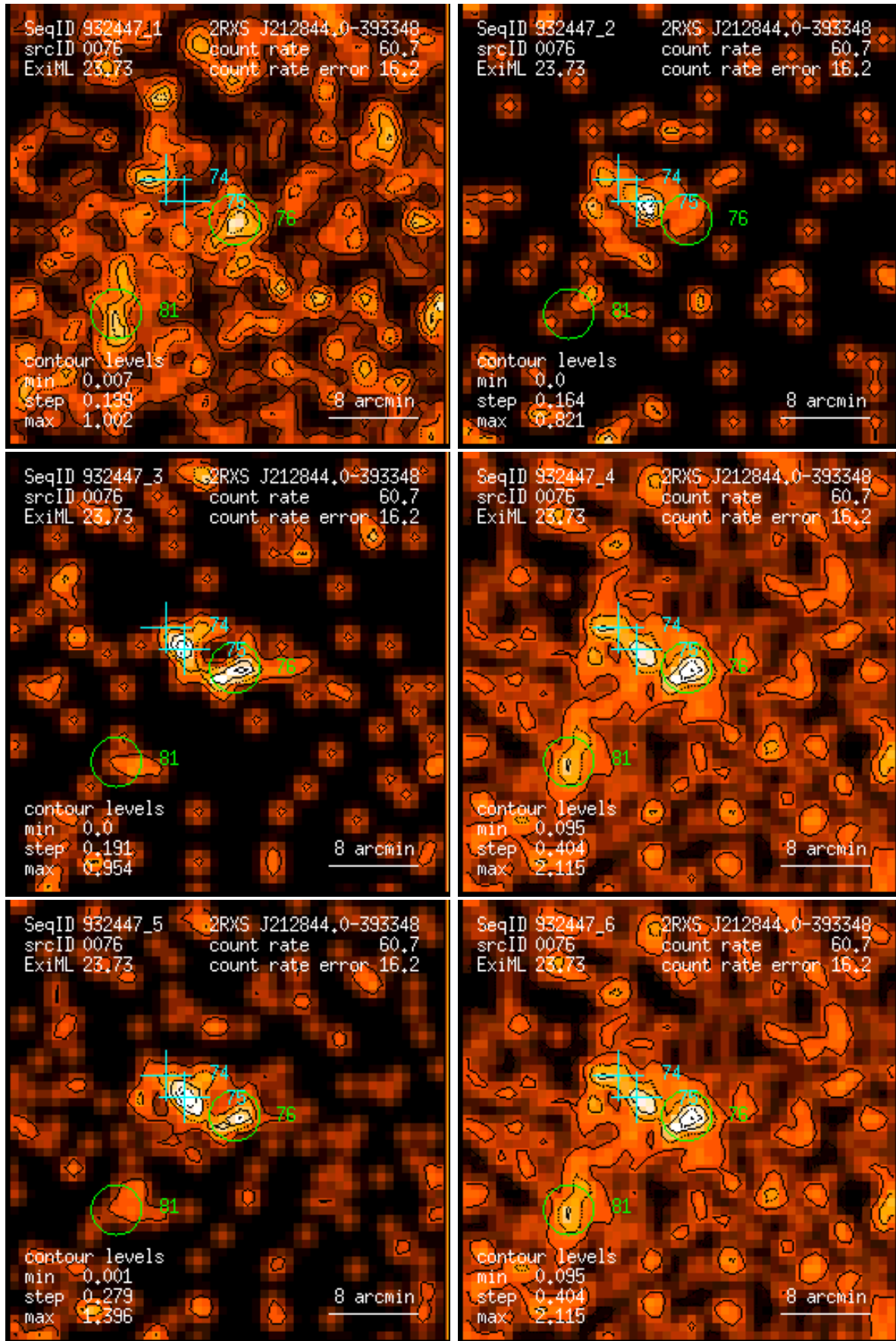
Figure 76: RASS 932447: detection 0076: band rate images, Gaussian filter: (1) PSPC channels 11 – 41, (2) 52 – 90, (3) 91 – 201, (4) 11 – 235, (5) 52 – 201, (6) 11 – 201. Broad band rates in counts/ks. Band rate contour levels in counts/ks/arcmin 2 .
