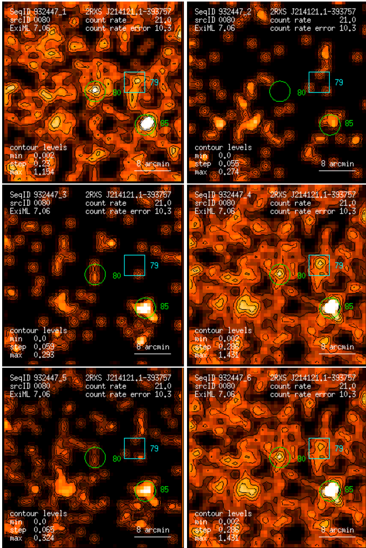
Figure 80: RASS 932447: detection 0080: band rate images, Gaussian filter: (1) PSPC channels 11 – 41, (2) 52 – 90, (3) 91 – 201, (4) 11 – 235, (5) 52 – 201, (6) 11 – 201. Broad band rates in counts/ks. Band rate contour levels in counts/ks/arcmin 2 .
