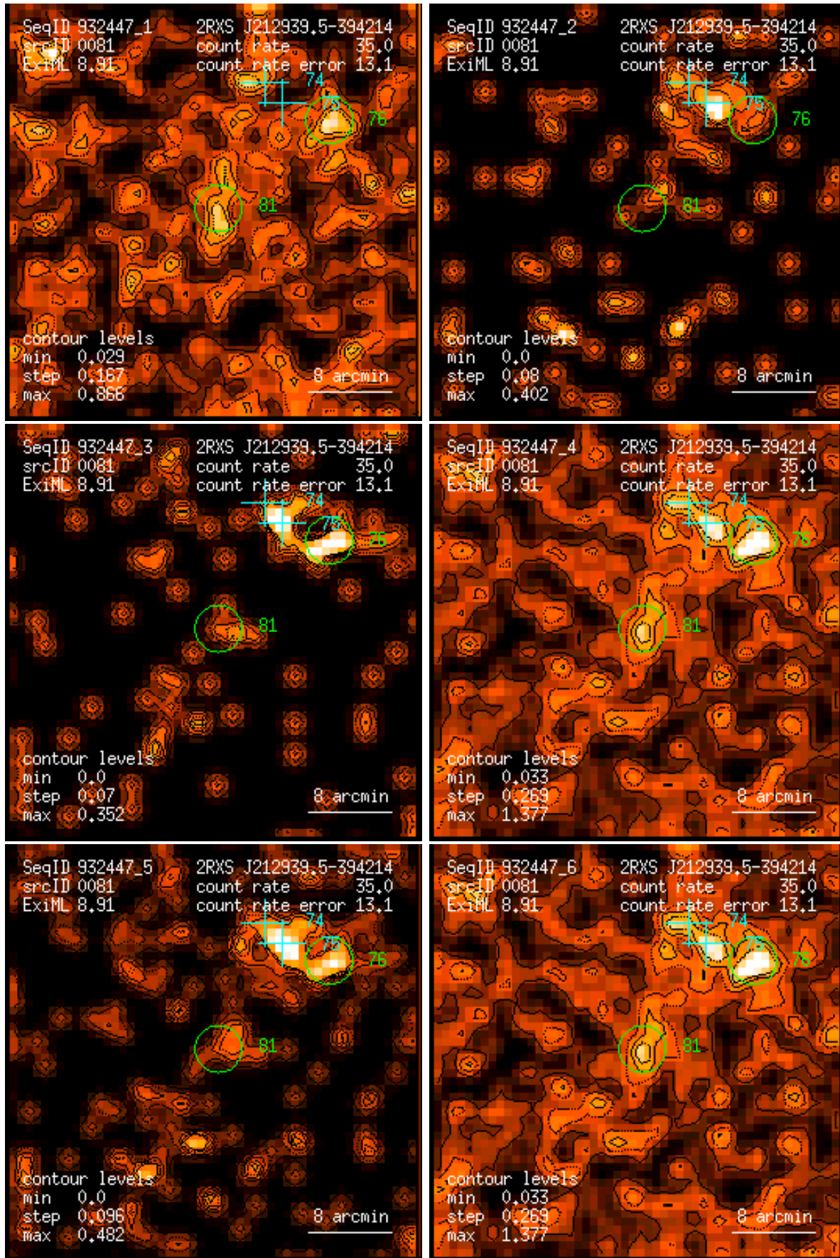
Figure 81: RASS 932447: detection 0081: band rate images, Gaussian filter: (1) PSPC channels 11 – 41, (2) 52 – 90, (3) 91 – 201, (4) 11 – 235, (5) 52 – 201, (6) 11 – 201. Broad band rates in counts/ks. Band rate contour levels in counts/ks/arcmin 2 .
