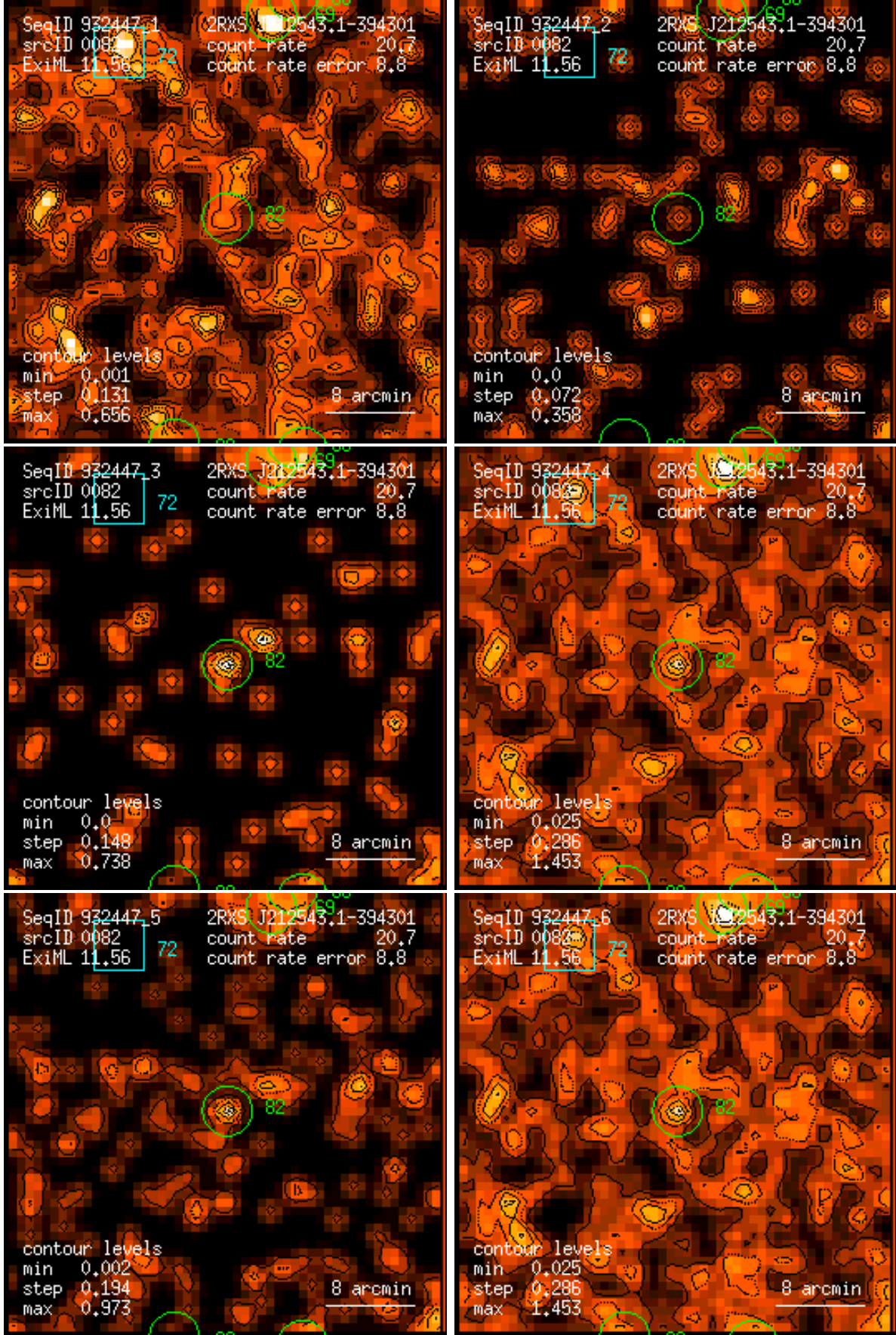
Figure 82: RASS 932447: detection 0082: band rate images, Gaussian filter: (1) PSPC channels 11 – 41, (2) 52 – 90, (3) 91 – 201, (4) 11 – 235, (5) 52 – 201, (6) 11 – 201. Broad band rates in counts/ks. Band rate contour levels in counts/ks/arcmin 2 .
