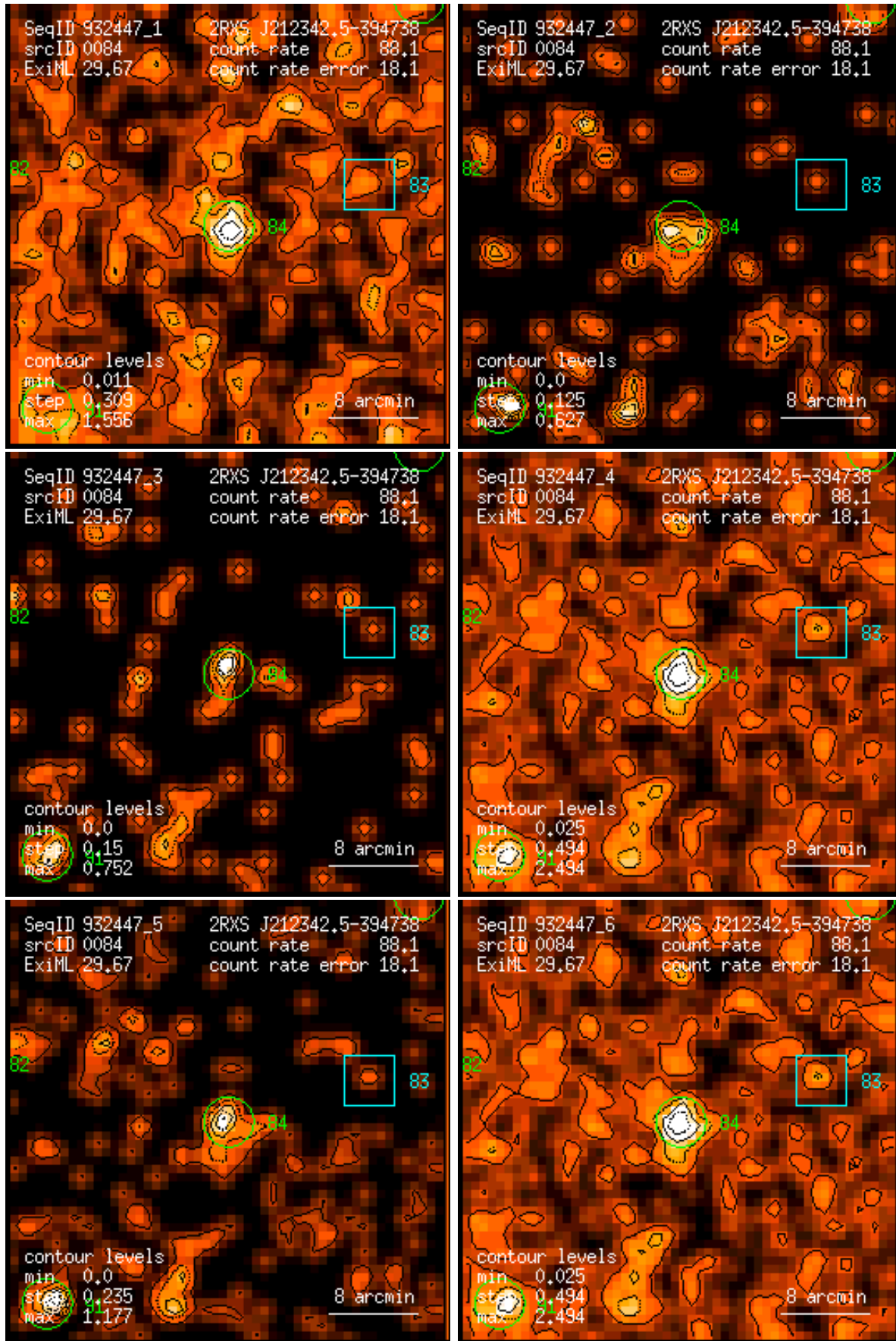
Figure 84: RASS 932447: detection 0084: band rate images, Gaussian filter: (1) PSPC channels 11 – 41, (2) 52 – 90, (3) 91 – 201, (4) 11 – 235, (5) 52 – 201, (6) 11 – 201. Broad band rates in counts/ks. Band rate contour levels in counts/ks/arcmin 2 .
