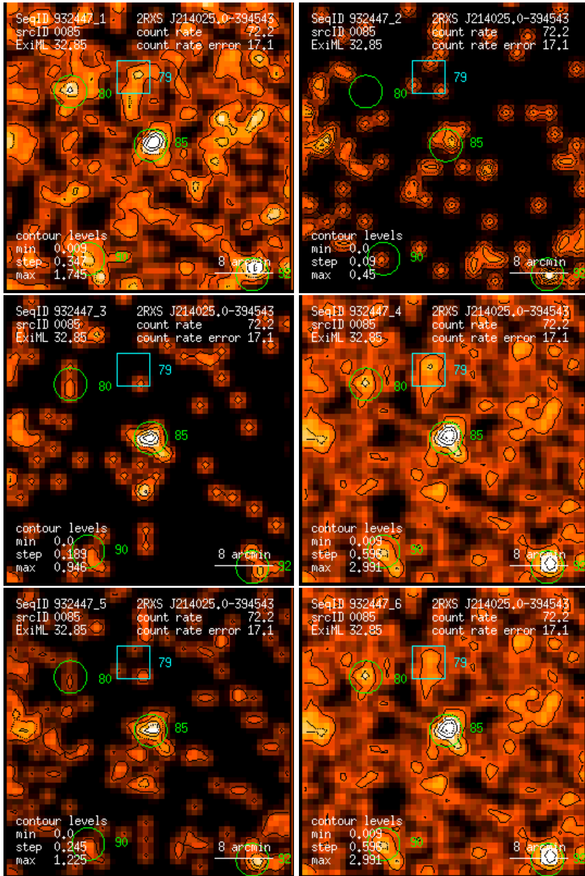
Figure 85: RASS 932447: detection 0085: band rate images, Gaussian filter: (1) PSPC channels 11 – 41, (2) 52 – 90, (3) 91 – 201, (4) 11 – 235, (5) 52 – 201, (6) 11 – 201. Broad band rates in counts/ks. Band rate contour levels in counts/ks/arcmin 2 .
