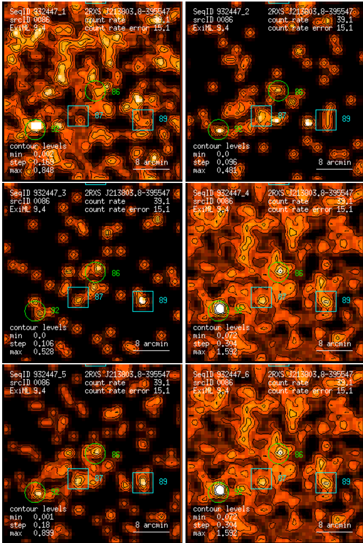
Figure 86: RASS 932447: detection 0086: band rate images, Gaussian filter: (1) PSPC channels 11 – 41, (2) 52 – 90, (3) 91 – 201, (4) 11 – 235, (5) 52 – 201, (6) 11 – 201. Broad band rates in counts/ks. Band rate contour levels in counts/ks/arcmin 2 .
