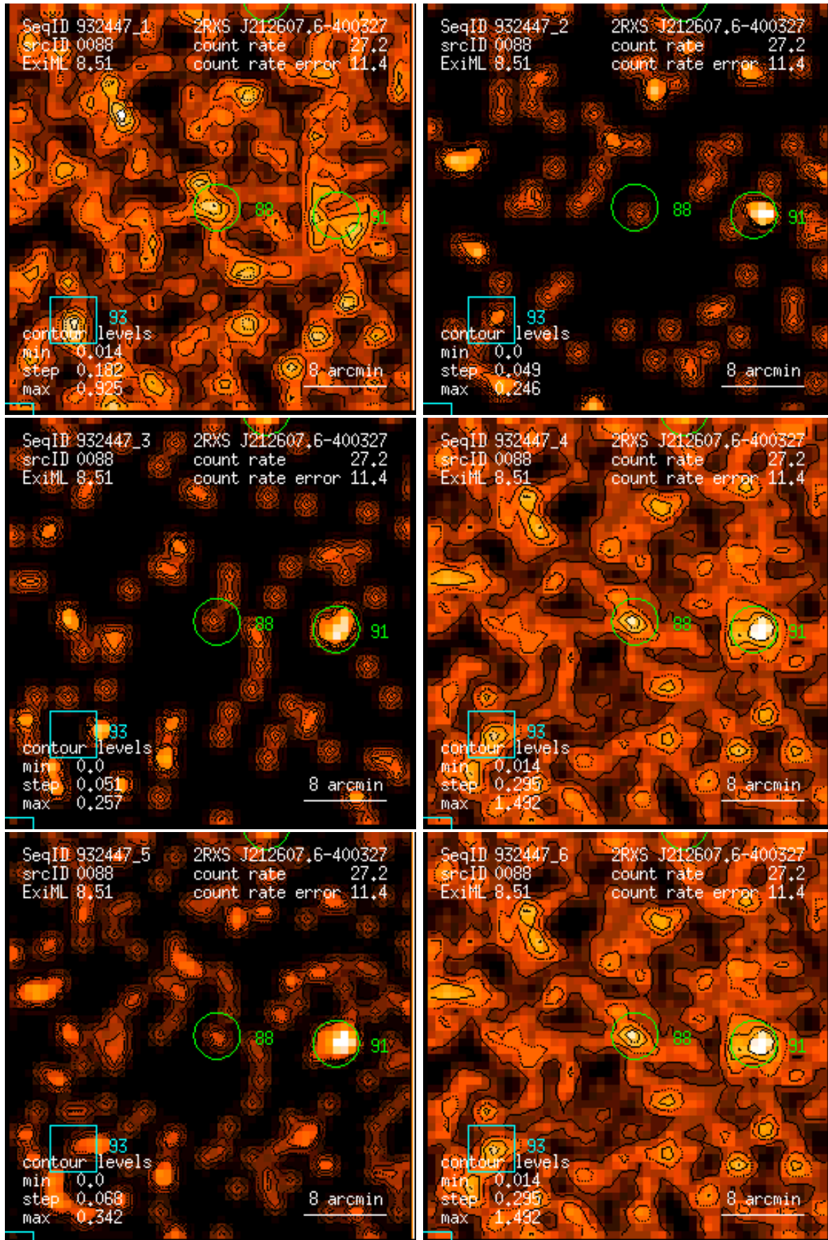
Figure 88: RASS 932447: detection 0088: band rate images, Gaussian filter: (1) PSPC channels 11 – 41, (2) 52 – 90, (3) 91 – 201, (4) 11 – 235, (5) 52 – 201, (6) 11 – 201. Broad band rates in counts/ks. Band rate contour levels in counts/ks/arcmin 2 .
