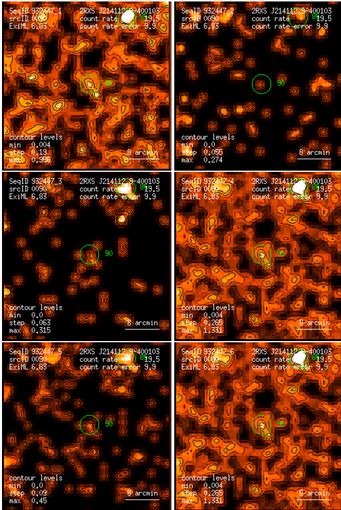
Figure 90: RASS 932447: detection 0090: band rate images, Gaussian filter: (1) PSPC channels 11 – 41, (2) 52 – 90, (3) 91 – 201, (4) 11 – 235, (5) 52 – 201, (6) 11 – 201. Broad band rates in counts/ks. Band rate contour levels in counts/ks/arcmin 2 .
