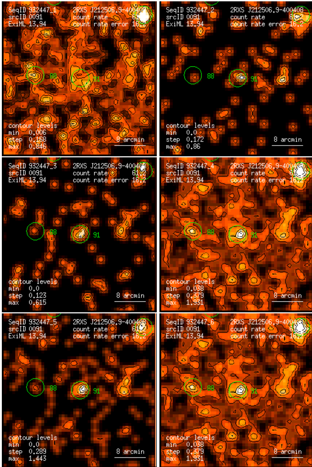
Figure 91: RASS 932447: detection 0091: band rate images, Gaussian filter: (1) PSPC channels 11 – 41, (2) 52 – 90, (3) 91 – 201, (4) 11 – 235, (5) 52 – 201, (6) 11 – 201. Broad band rates in counts/ks. Band rate contour levels in counts/ks/arcmin 2 .
