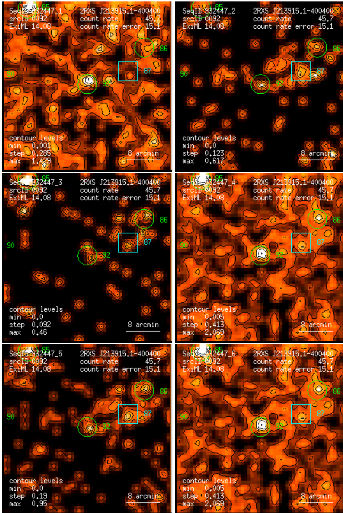
Figure 92: RASS 932447: detection 0092: band rate images, Gaussian filter: (1) PSPC channels 11 – 41, (2) 52 – 90, (3) 91 – 201, (4) 11 – 235, (5) 52 – 201, (6) 11 – 201. Broad band rates in counts/ks. Band rate contour levels in counts/ks/arcmin 2 .
