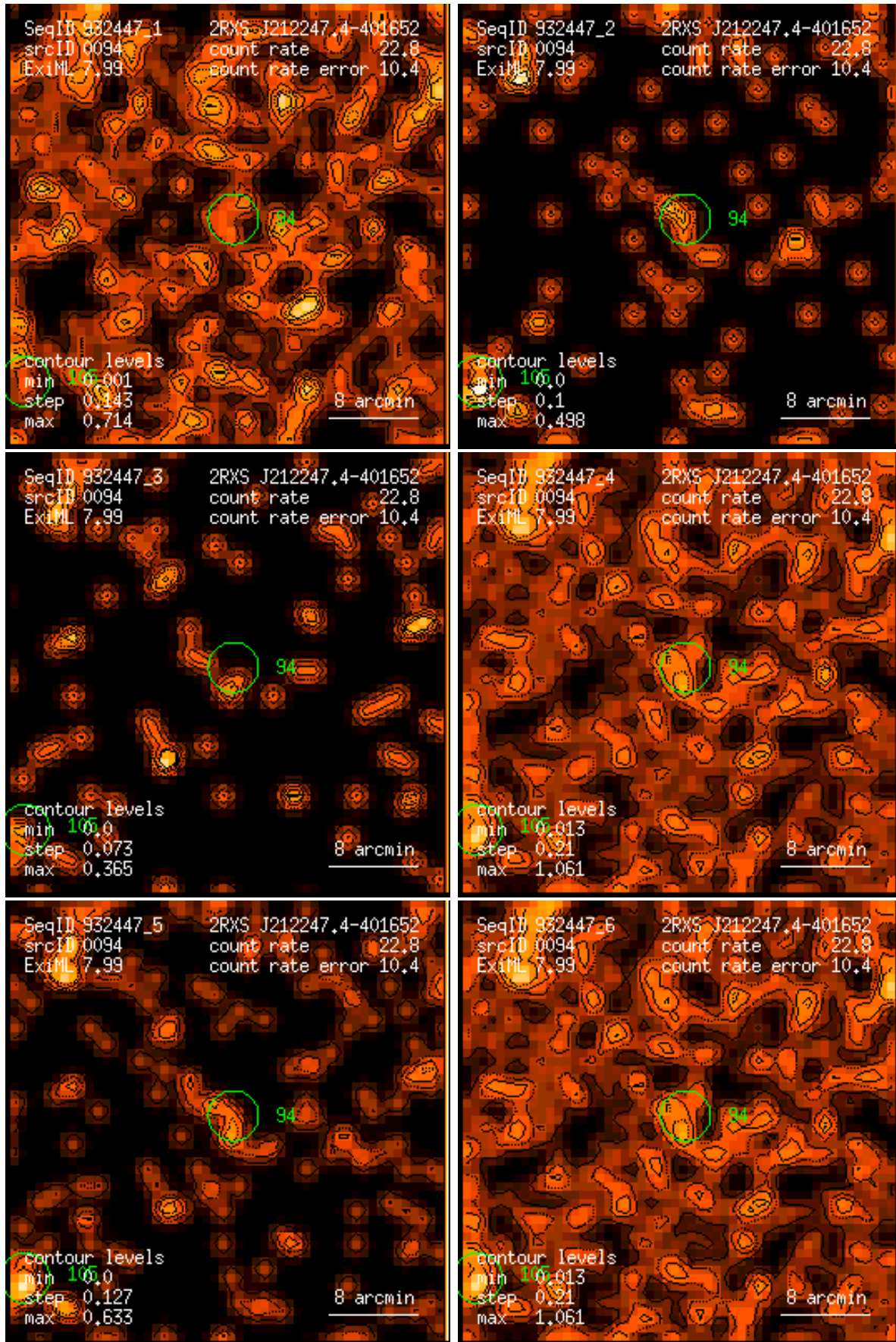
Figure 94: RASS 932447: detection 0094: band rate images, Gaussian filter: (1) PSPC channels 11 – 41, (2) 52 – 90, (3) 91 – 201, (4) 11 – 235, (5) 52 – 201, (6) 11 – 201. Broad band rates in counts/ks. Band rate contour levels in counts/ks/arcmin 2 .
