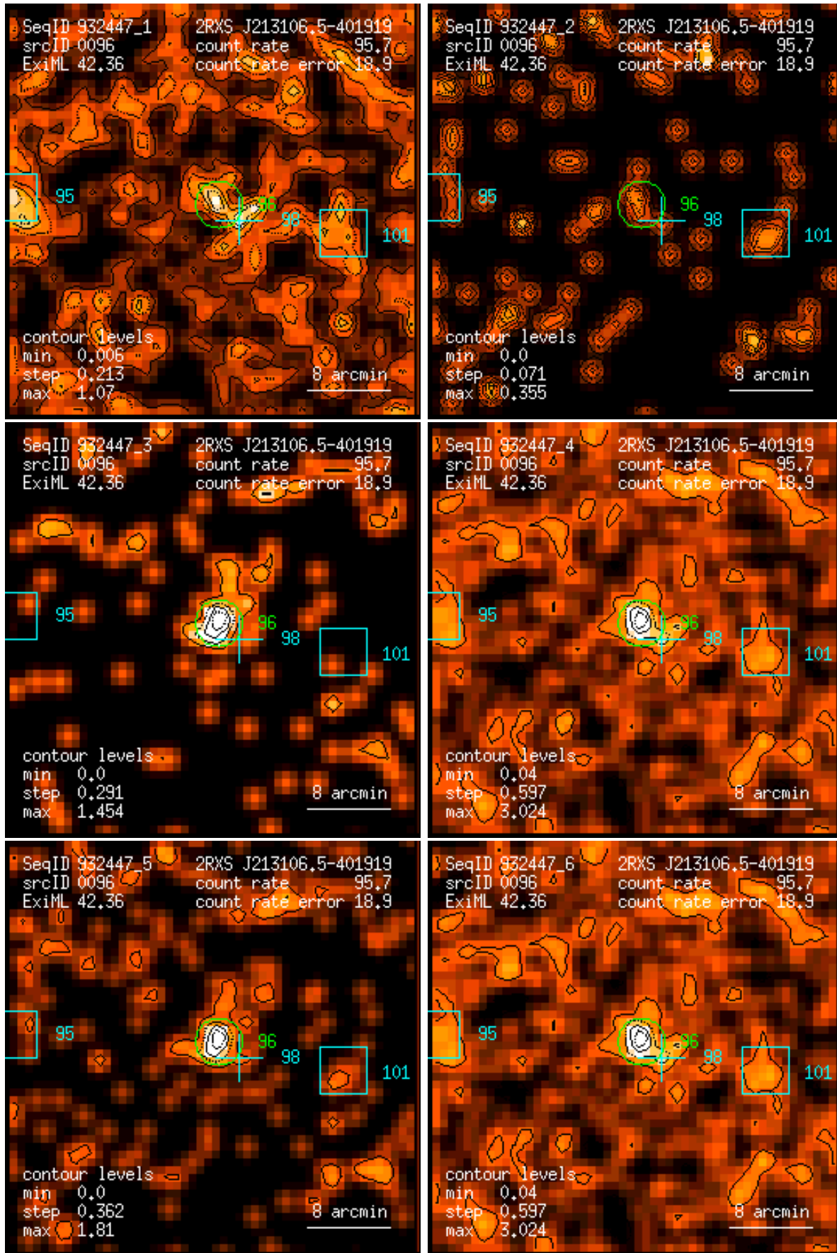
Figure 96: RASS 932447: detection 0096: band rate images, Gaussian filter: (1) PSPC channels 11 – 41, (2) 52 – 90, (3) 91 – 201, (4) 11 – 235, (5) 52 – 201, (6) 11 – 201. Broad band rates in counts/ks. Band rate contour levels in counts/ks/arcmin 2 .
