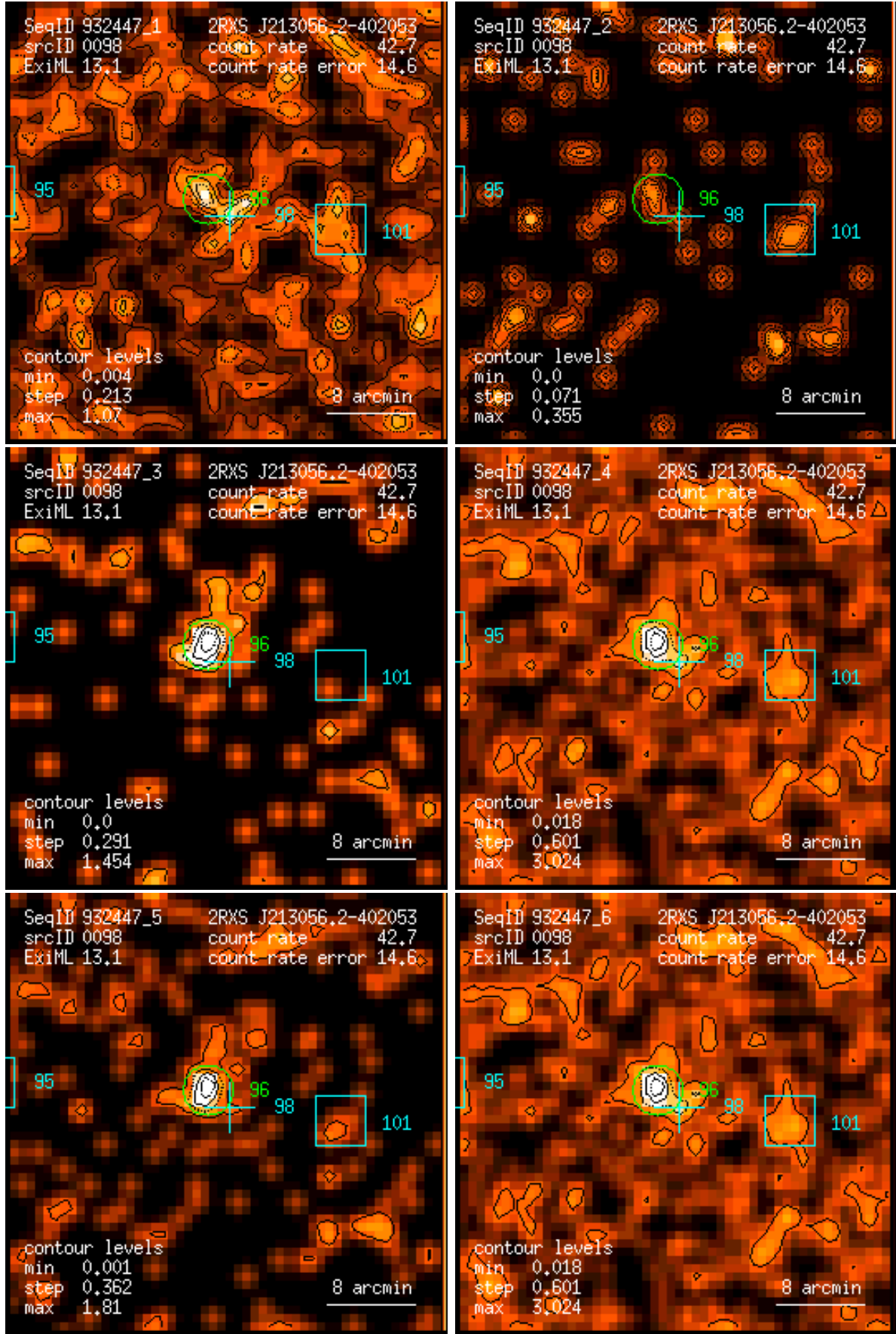
Figure 98: RASS 932447: detection 0098: band rate images, Gaussian filter: (1) PSPC channels 11 – 41, (2) 52 – 90, (3) 91 – 201, (4) 11 – 235, (5) 52 – 201, (6) 11 – 201. Broad band rates in counts/ks. Band rate contour levels in counts/ks/arcmin 2 .
