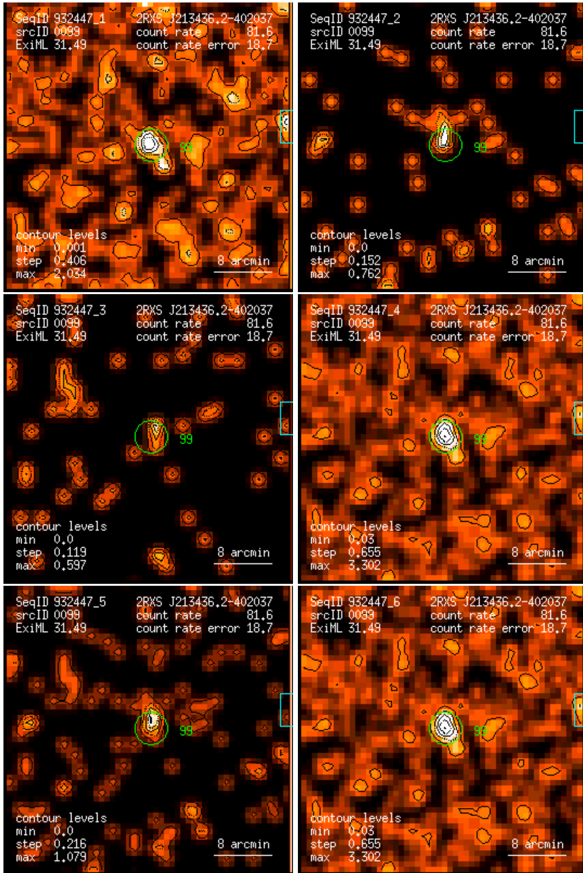
Figure 99: RASS 932447: detection 0099: band rate images, Gaussian filter: (1) PSPC channels 11 – 41, (2) 52 – 90, (3) 91 – 201, (4) 11 – 235, (5) 52 – 201, (6) 11 – 201. Broad band rates in counts/ks. Band rate contour levels in counts/ks/arcmin 2 .
