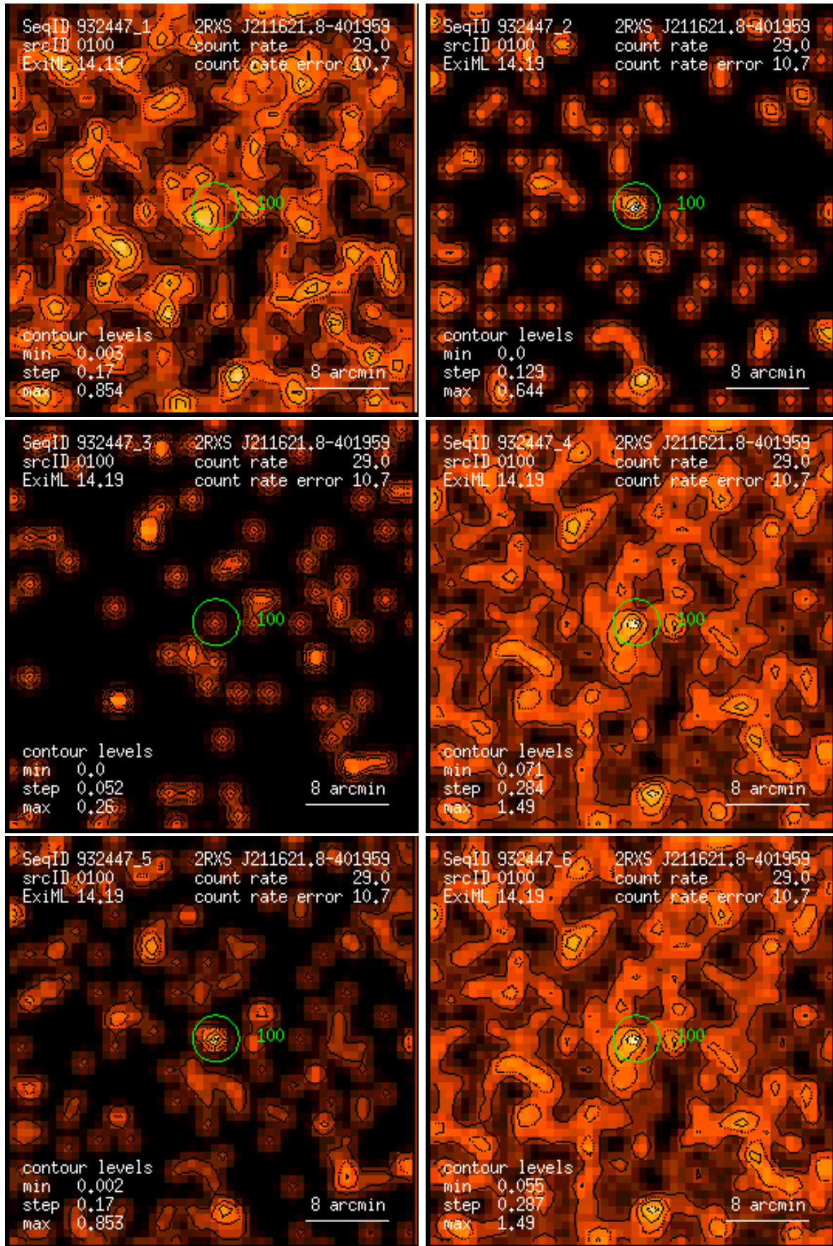
Figure 100: RASS 932447: detection 0100: band rate images, Gaussian filter: (1) PSPC channels 11 – 41, (2) 52 – 90, (3) 91 – 201, (4) 11 – 235, (5) 52 – 201, (6) 11 – 201. Broad band rates in counts/ks. Band rate contour levels in counts/ks/arcmin 2 .
