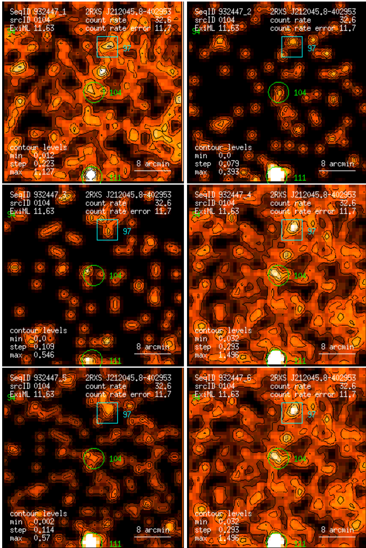
Figure 104: RASS 932447: detection 0104: band rate images, Gaussian filter: (1) PSPC channels 11 – 41, (2) 52 – 90, (3) 91 – 201, (4) 11 – 235, (5) 52 – 201, (6) 11 – 201. Broad band rates in counts/ks. Band rate contour levels in counts/ks/arcmin 2 .
