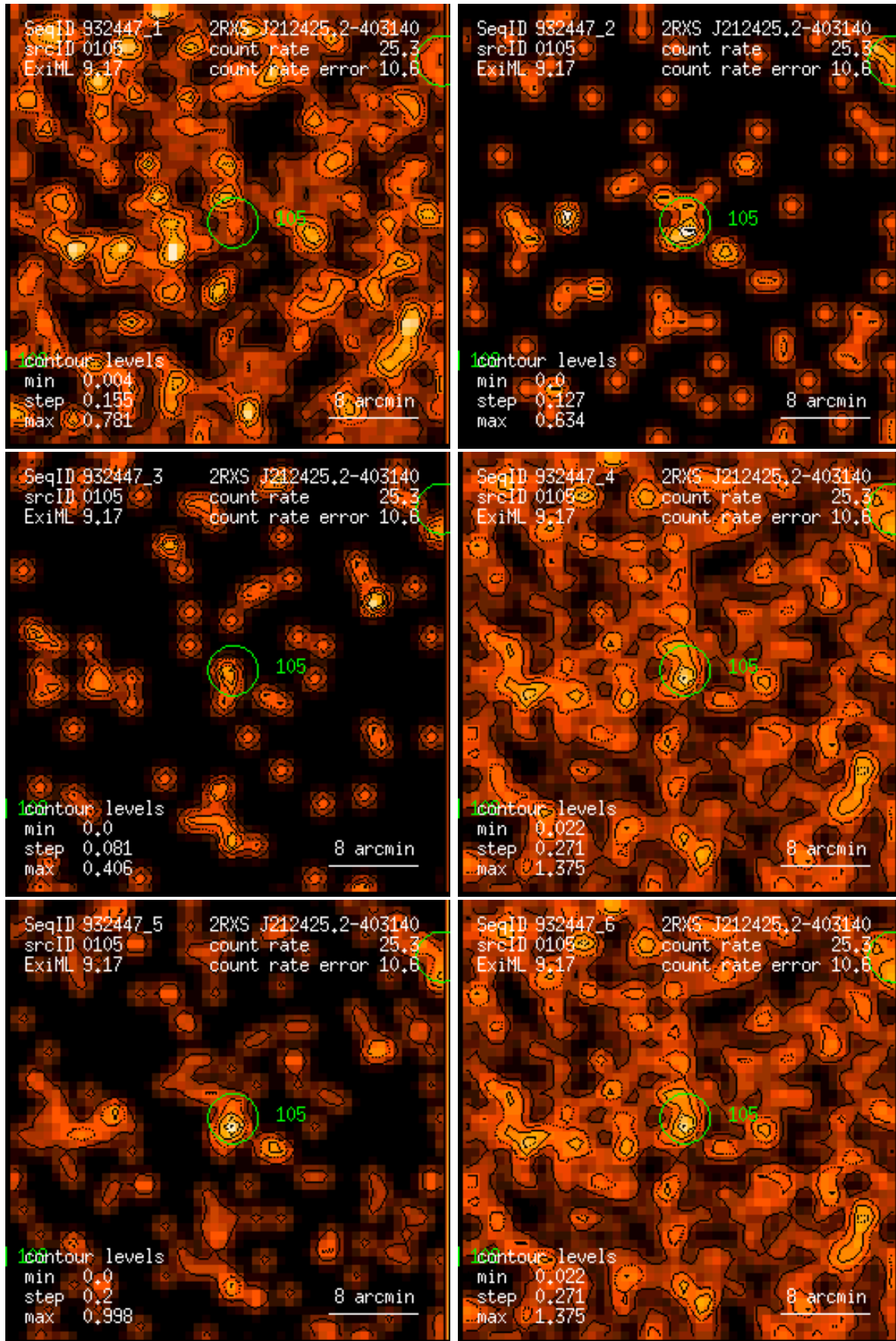
Figure 105: RASS 932447: detection 0105: band rate images, Gaussian filter: (1) PSPC channels 11 – 41, (2) 52 – 90, (3) 91 – 201, (4) 11 – 235, (5) 52 – 201, (6) 11 – 201. Broad band rates in counts/ks. Band rate contour levels in counts/ks/arcmin 2 .
