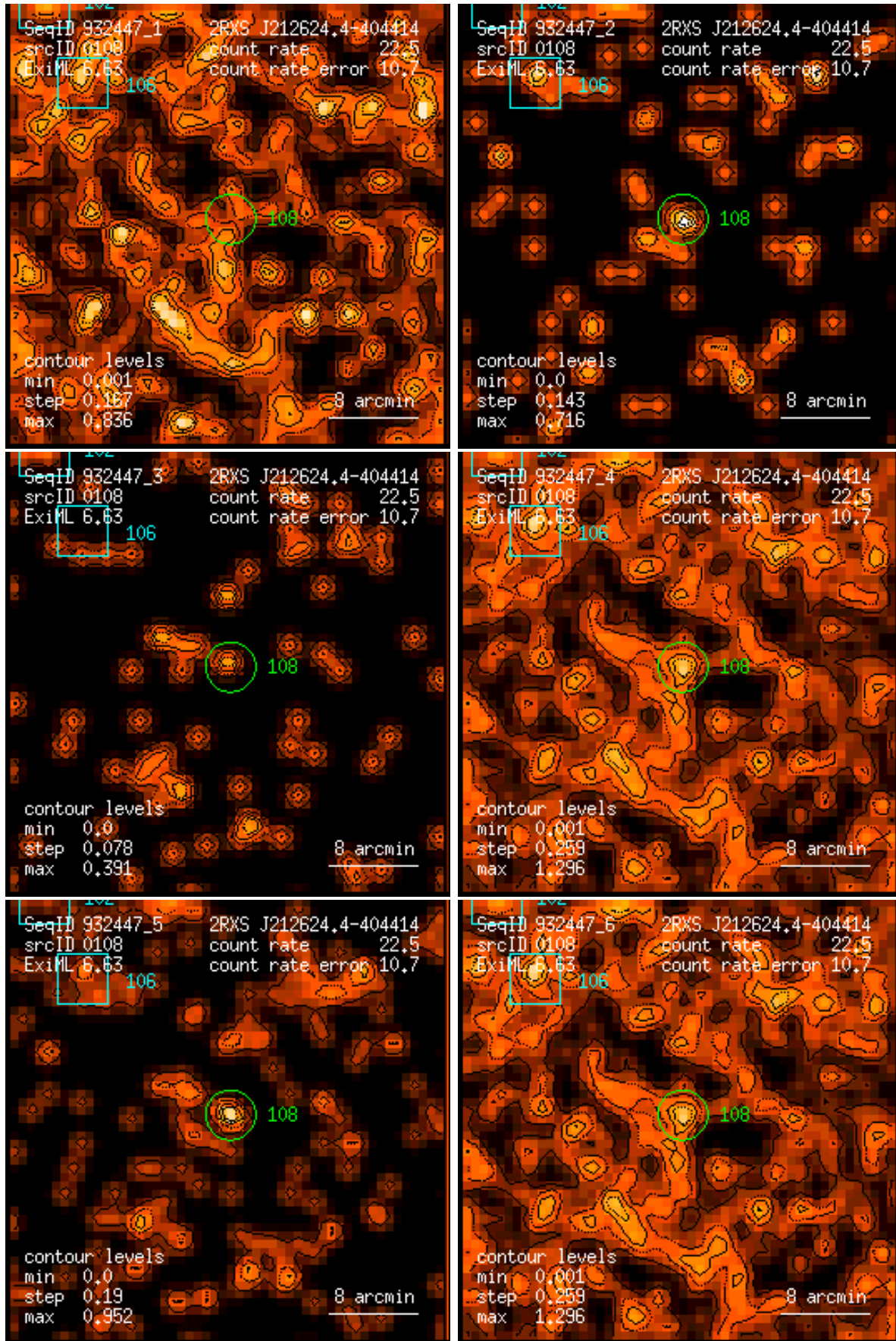
Figure 108: RASS 932447: detection 0108: band rate images, Gaussian filter: (1) PSPC channels 11 – 41, (2) 52 – 90, (3) 91 – 201, (4) 11 – 235, (5) 52 – 201, (6) 11 – 201. Broad band rates in counts/ks. Band rate contour levels in counts/ks/arcmin 2 .
