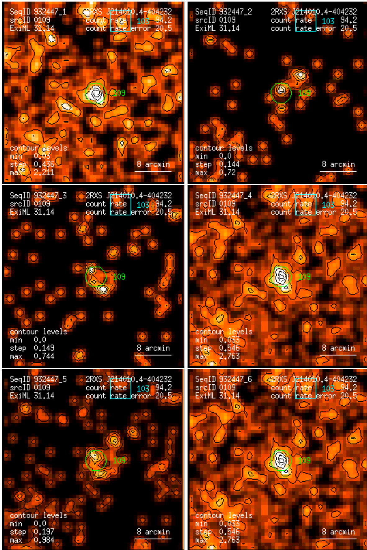
Figure 109: RASS 932447: detection 0109: band rate images, Gaussian filter: (1) PSPC channels 11 – 41, (2) 52 – 90, (3) 91 – 201, (4) 11 – 235, (5) 52 – 201, (6) 11 – 201. Broad band rates in counts/ks. Band rate contour levels in counts/ks/arcmin 2 .
