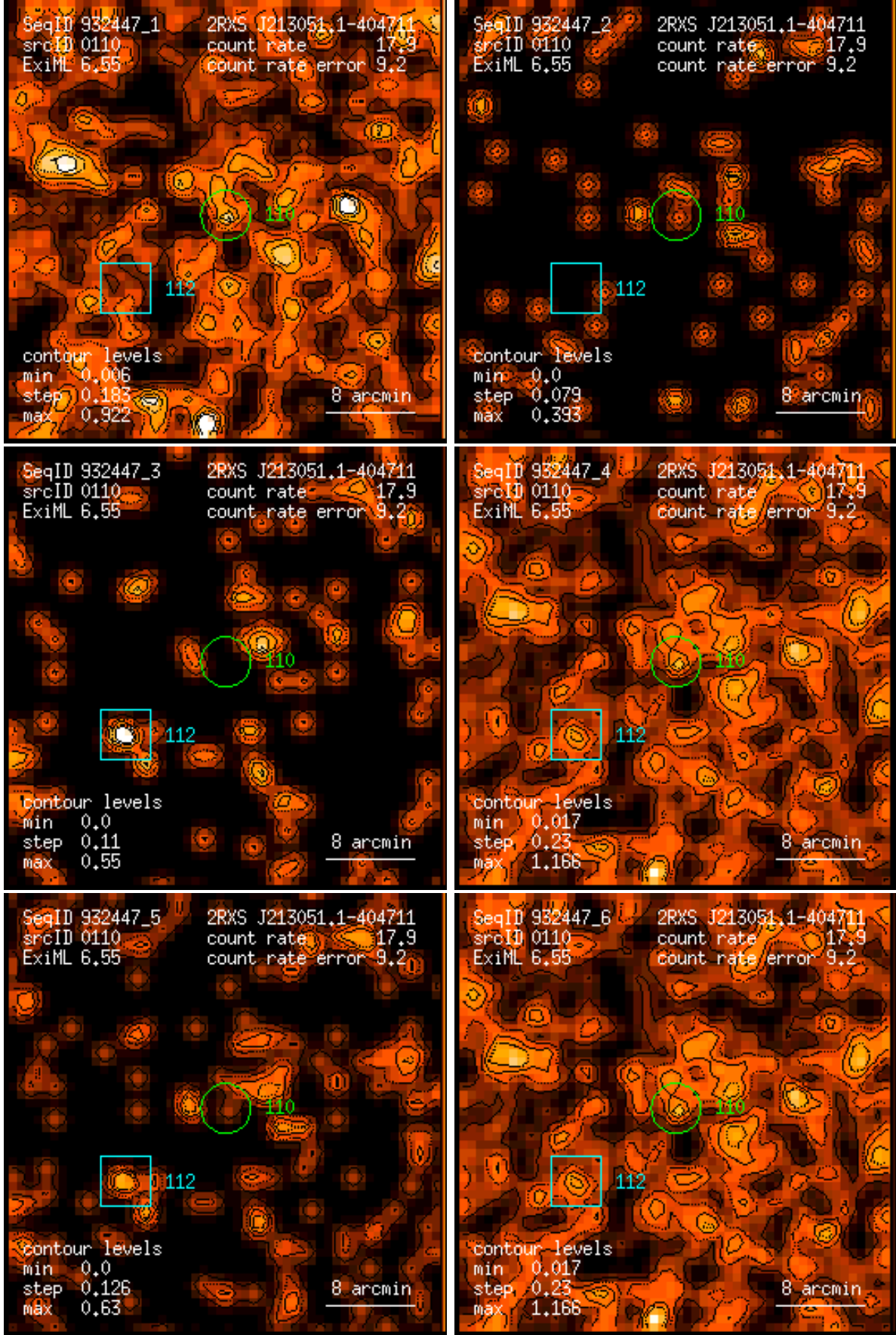
Figure 110: RASS 932447: detection 0110: band rate images, Gaussian filter: (1) PSPC channels 11 – 41, (2) 52 – 90, (3) 91 – 201, (4) 11 – 235, (5) 52 – 201, (6) 11 – 201. Broad band rates in counts/ks. Band rate contour levels in counts/ks/arcmin 2 .
