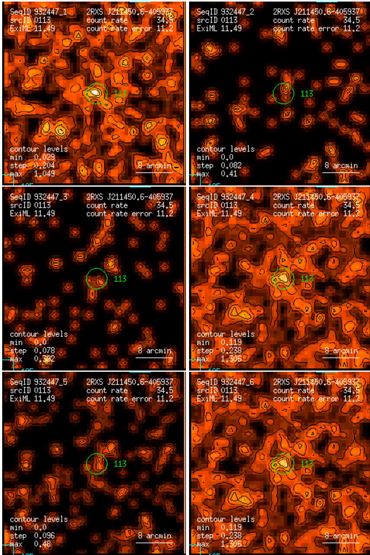
Figure 113: RASS 932447: detection 0113: band rate images, Gaussian filter: (1) PSPC channels 11 – 41, (2) 52 – 90, (3) 91 – 201, (4) 11 – 235, (5) 52 – 201, (6) 11 – 201. Broad band rates in counts/ks. Band rate contour levels in counts/ks/arcmin 2 .
