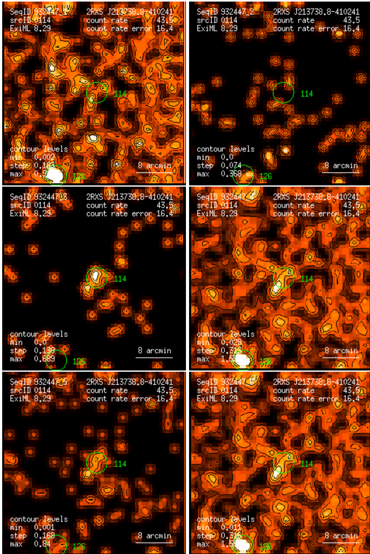
Figure 114: RASS 932447: detection 0114: band rate images, Gaussian filter: (1) PSPC channels 11 – 41, (2) 52 – 90, (3) 91 – 201, (4) 11 – 235, (5) 52 – 201, (6) 11 – 201. Broad band rates in counts/ks. Band rate contour levels in counts/ks/arcmin 2 .
