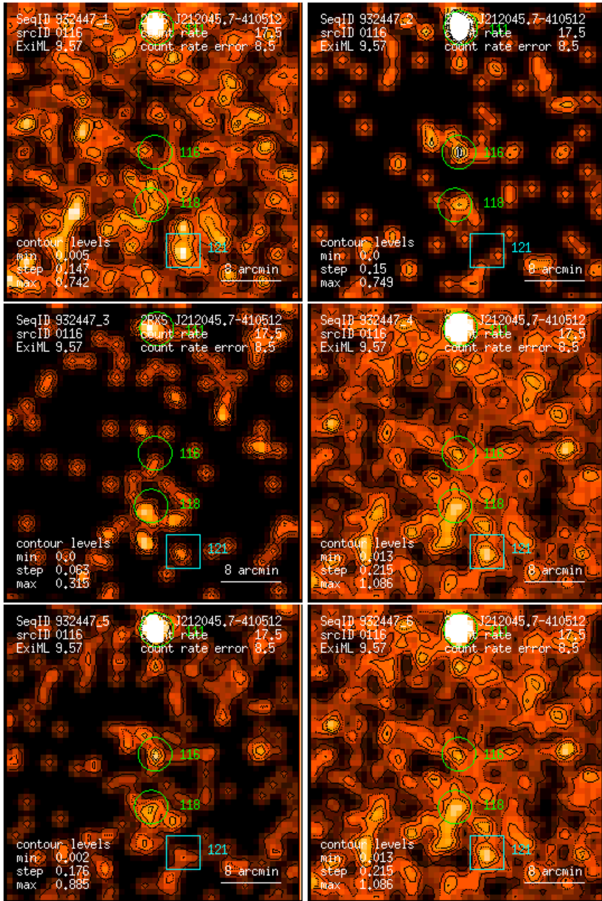
Figure 116: RASS 932447: detection 0116: band rate images, Gaussian filter: (1) PSPC channels 11 – 41, (2) 52 – 90, (3) 91 – 201, (4) 11 – 235, (5) 52 – 201, (6) 11 – 201. Broad band rates in counts/ks. Band rate contour levels in counts/ks/arcmin 2 .
