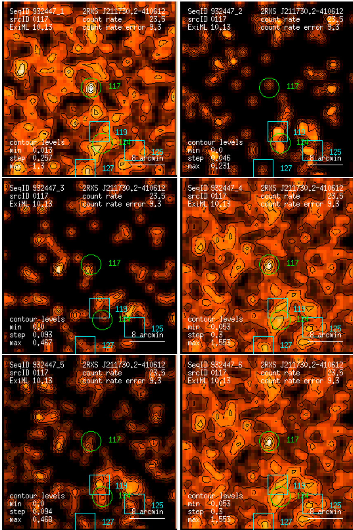
Figure 117: RASS 932447: detection 0117: band rate images, Gaussian filter: (1) PSPC channels 11 – 41, (2) 52 – 90, (3) 91 – 201, (4) 11 – 235, (5) 52 – 201, (6) 11 – 201. Broad band rates in counts/ks. Band rate contour levels in counts/ks/arcmin 2 .
