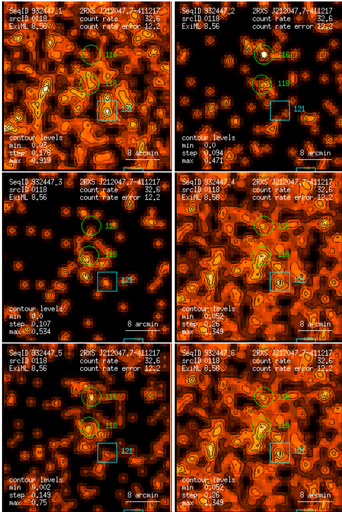
Figure 118: RASS 932447: detection 0118: band rate images, Gaussian filter: (1) PSPC channels 11 – 41, (2) 52 – 90, (3) 91 – 201, (4) 11 – 235, (5) 52 – 201, (6) 11 – 201. Broad band rates in counts/ks. Band rate contour levels in counts/ks/arcmin 2 .
