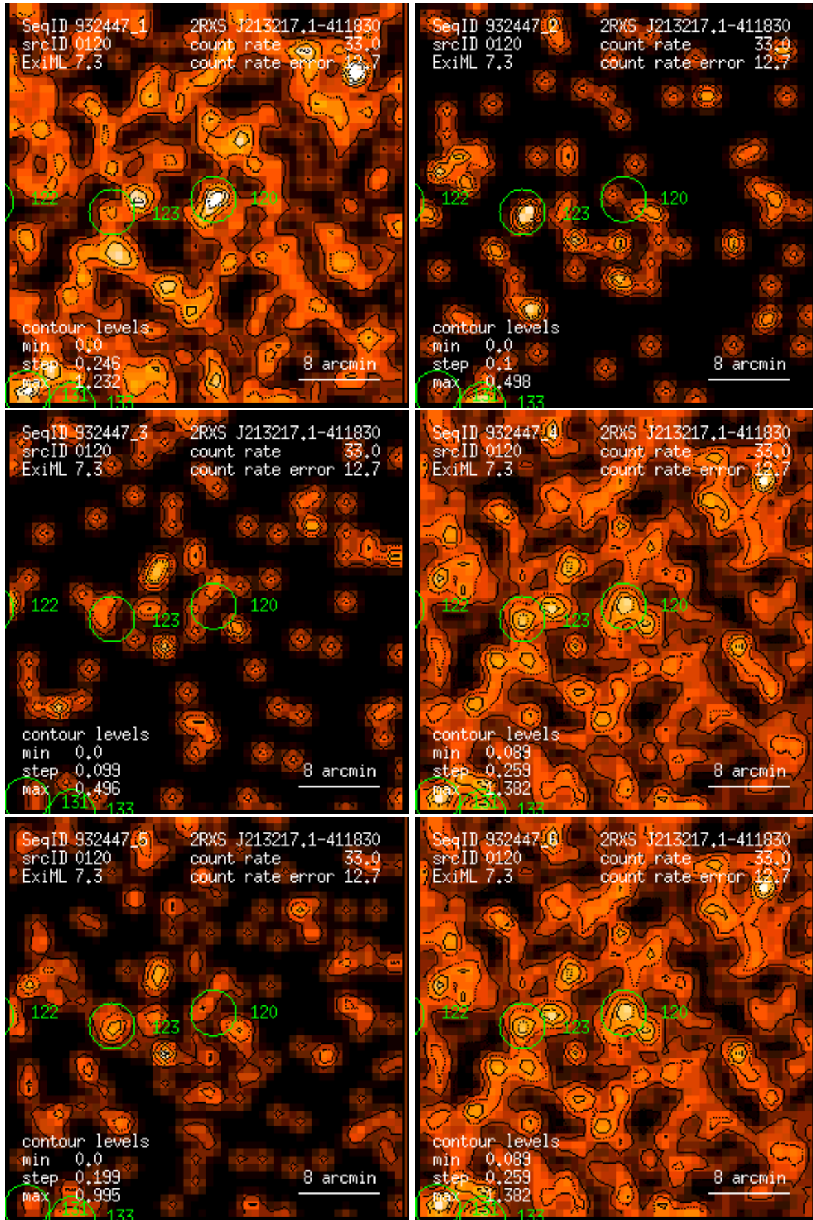
Figure 120: RASS 932447: detection 0120: band rate images, Gaussian filter: (1) PSPC channels 11 – 41, (2) 52 – 90, (3) 91 – 201, (4) 11 – 235, (5) 52 – 201, (6) 11 – 201. Broad band rates in counts/ks. Band rate contour levels in counts/ks/arcmin 2 .
