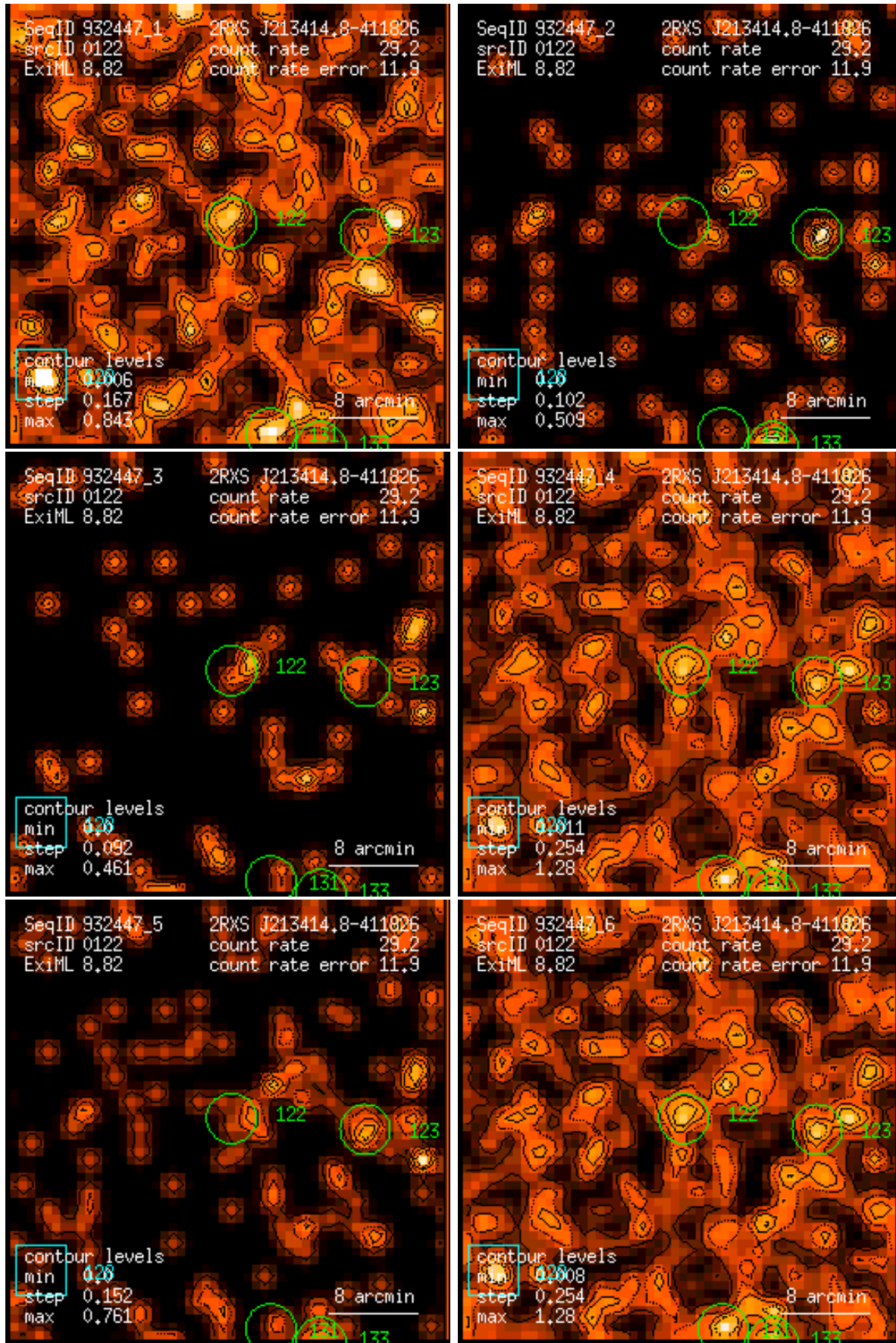
Figure 122: RASS 932447: detection 0122: band rate images, Gaussian filter: (1) PSPC channels 11 – 41, (2) 52 – 90, (3) 91 – 201, (4) 11 – 235, (5) 52 – 201, (6) 11 – 201. Broad band rates in counts/ks. Band rate contour levels in counts/ks/arcmin 2 .
