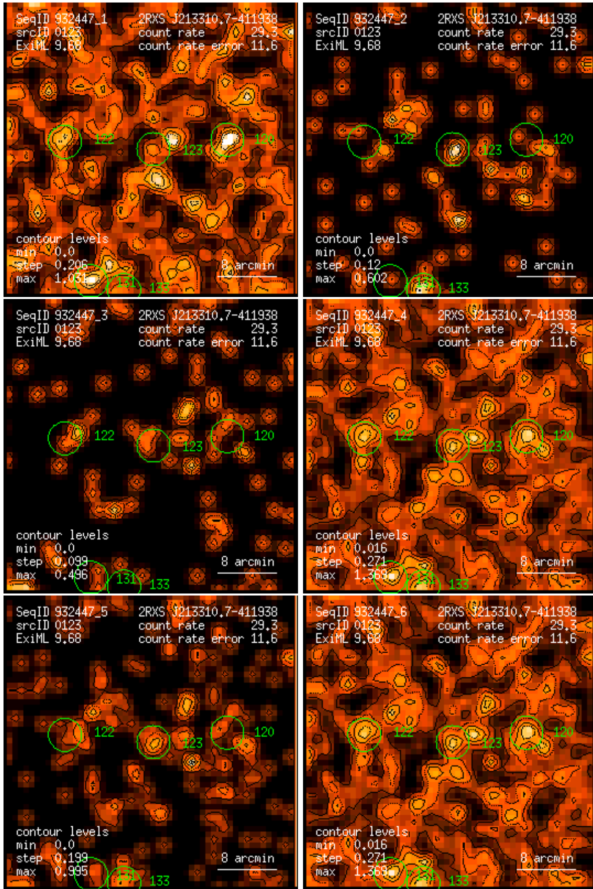
Figure 123: RASS 932447: detection 0123: band rate images, Gaussian filter: (1) PSPC channels 11 – 41, (2) 52 – 90, (3) 91 – 201, (4) 11 – 235, (5) 52 – 201, (6) 11 – 201. Broad band rates in counts/ks. Band rate contour levels in counts/ks/arcmin 2 .
