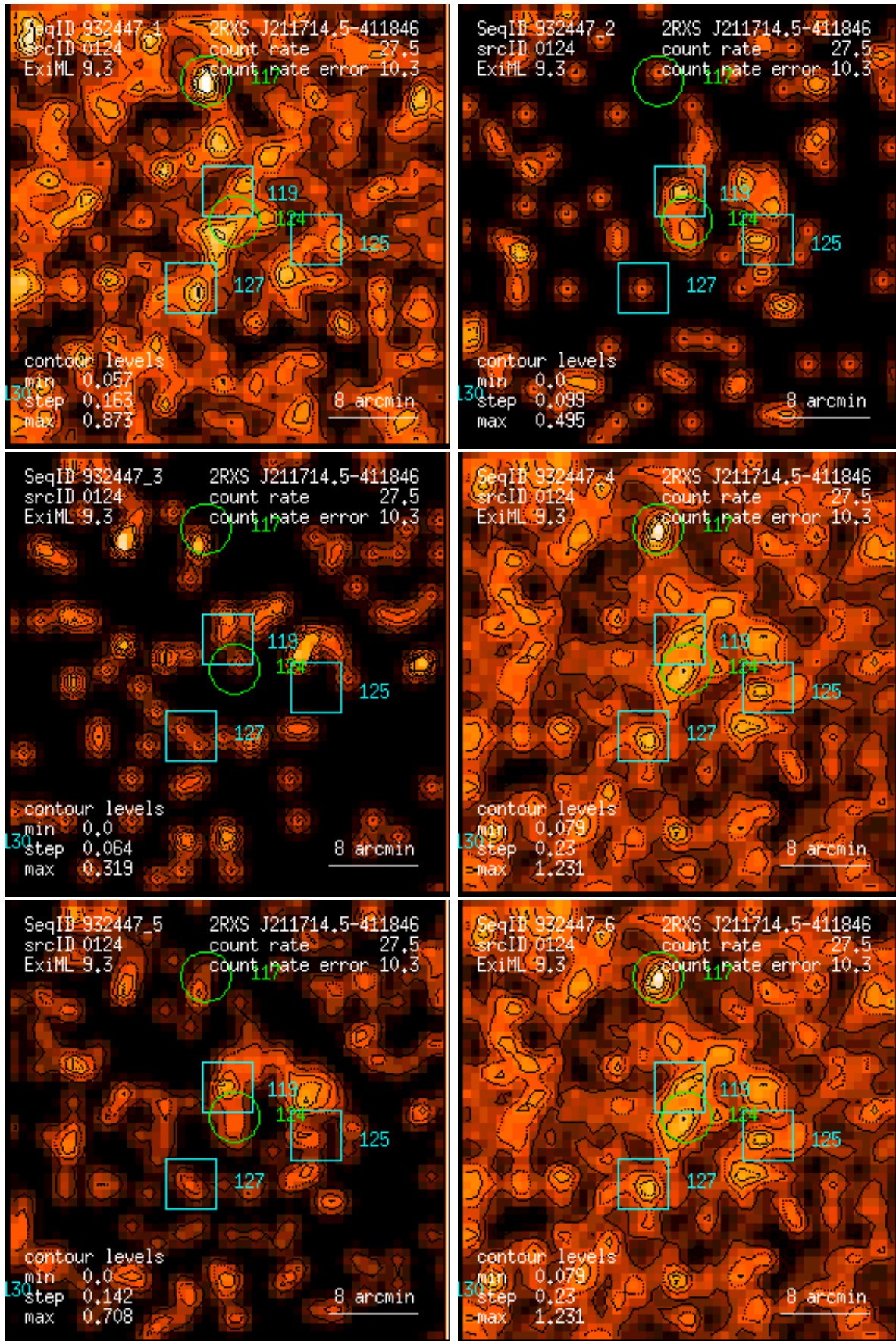
Figure 124: RASS 932447: detection 0124: band rate images, Gaussian filter: (1) PSPC channels 11 – 41, (2) 52 – 90, (3) 91 – 201, (4) 11 – 235, (5) 52 – 201, (6) 11 – 201. Broad band rates in counts/ks. Band rate contour levels in counts/ks/arcmin 2 .
