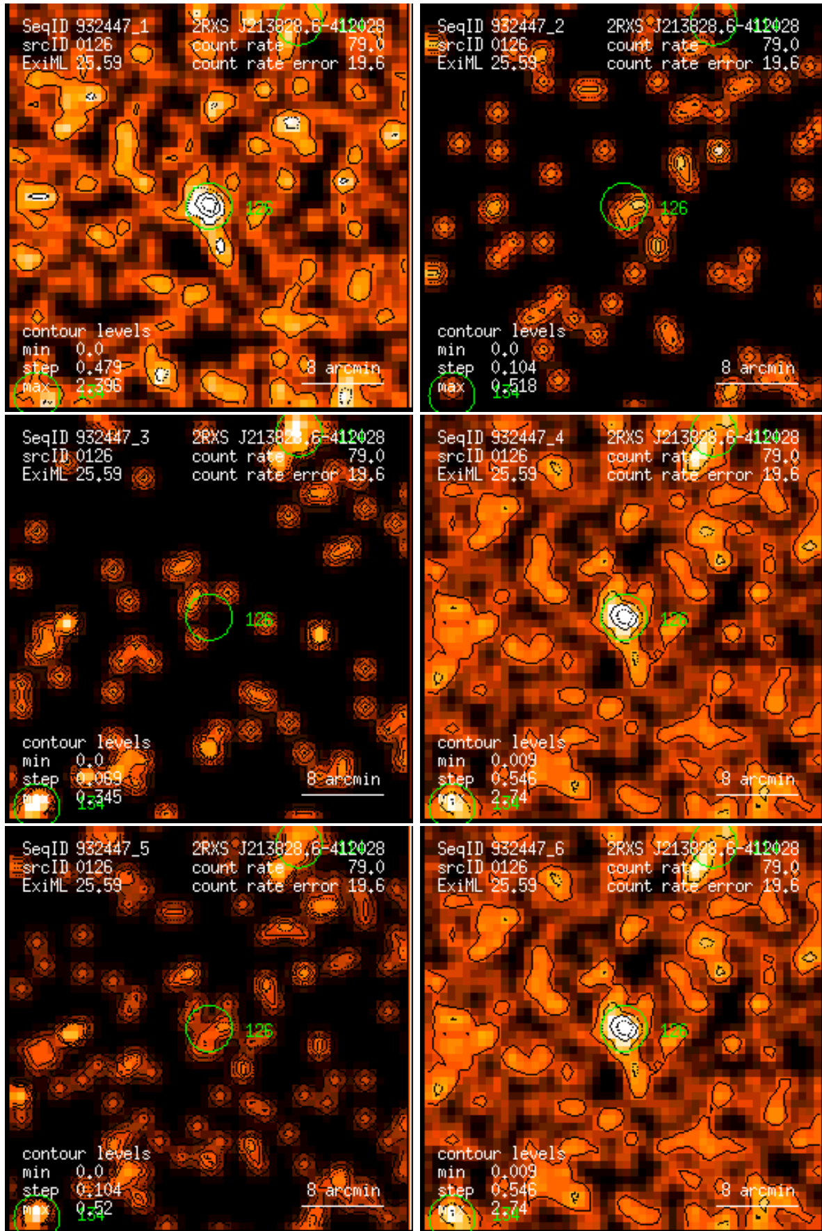
Figure 126: RASS 932447: detection 0126: band rate images, Gaussian filter: (1) PSPC channels 11 – 41, (2) 52 – 90, (3) 91 – 201, (4) 11 – 235, (5) 52 – 201, (6) 11 – 201. Broad band rates in counts/ks. Band rate contour levels in counts/ks/arcmin 2 .
