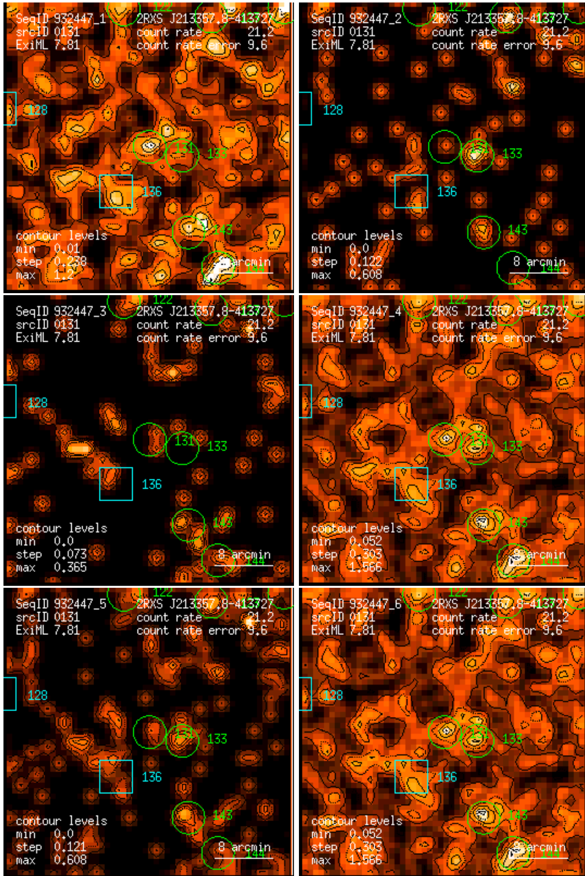
Figure 131: RASS 932447: detection 0131: band rate images, Gaussian filter: (1) PSPC channels 11 – 41, (2) 52 – 90, (3) 91 – 201, (4) 11 – 235, (5) 52 – 201, (6) 11 – 201. Broad band rates in counts/ks. Band rate contour levels in counts/ks/arcmin 2 .
