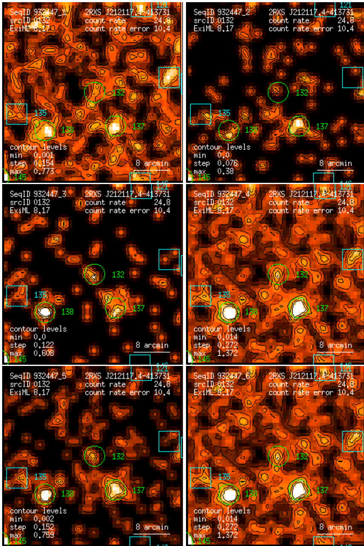
Figure 132: RASS 932447: detection 0132: band rate images, Gaussian filter: (1) PSPC channels 11 – 41, (2) 52 – 90, (3) 91 – 201, (4) 11 – 235, (5) 52 – 201, (6) 11 – 201. Broad band rates in counts/ks. Band rate contour levels in counts/ks/arcmin 2 .
