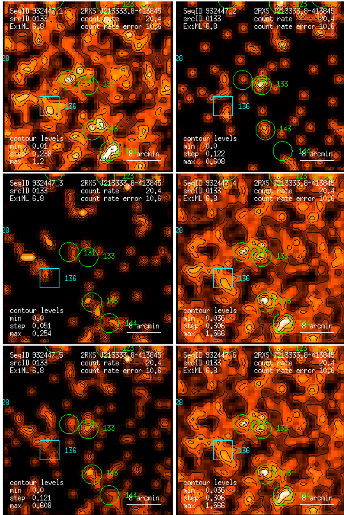
Figure 133: RASS 932447: detection 0133: band rate images, Gaussian filter: (1) PSPC channels 11 – 41, (2) 52 – 90, (3) 91 – 201, (4) 11 – 235, (5) 52 – 201, (6) 11 – 201. Broad band rates in counts/ks. Band rate contour levels in counts/ks/arcmin 2 .
