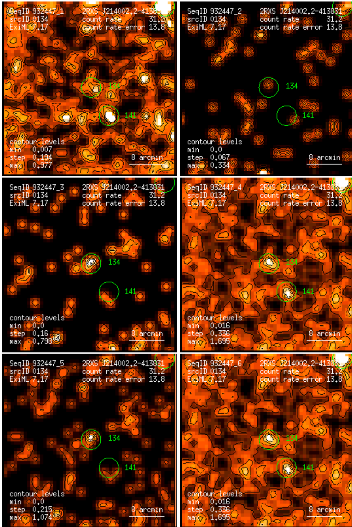
Figure 134: RASS 932447: detection 0134: band rate images, Gaussian filter: (1) PSPC channels 11 – 41, (2) 52 – 90, (3) 91 – 201, (4) 11 – 235, (5) 52 – 201, (6) 11 – 201. Broad band rates in counts/ks. Band rate contour levels in counts/ks/arcmin 2 .
