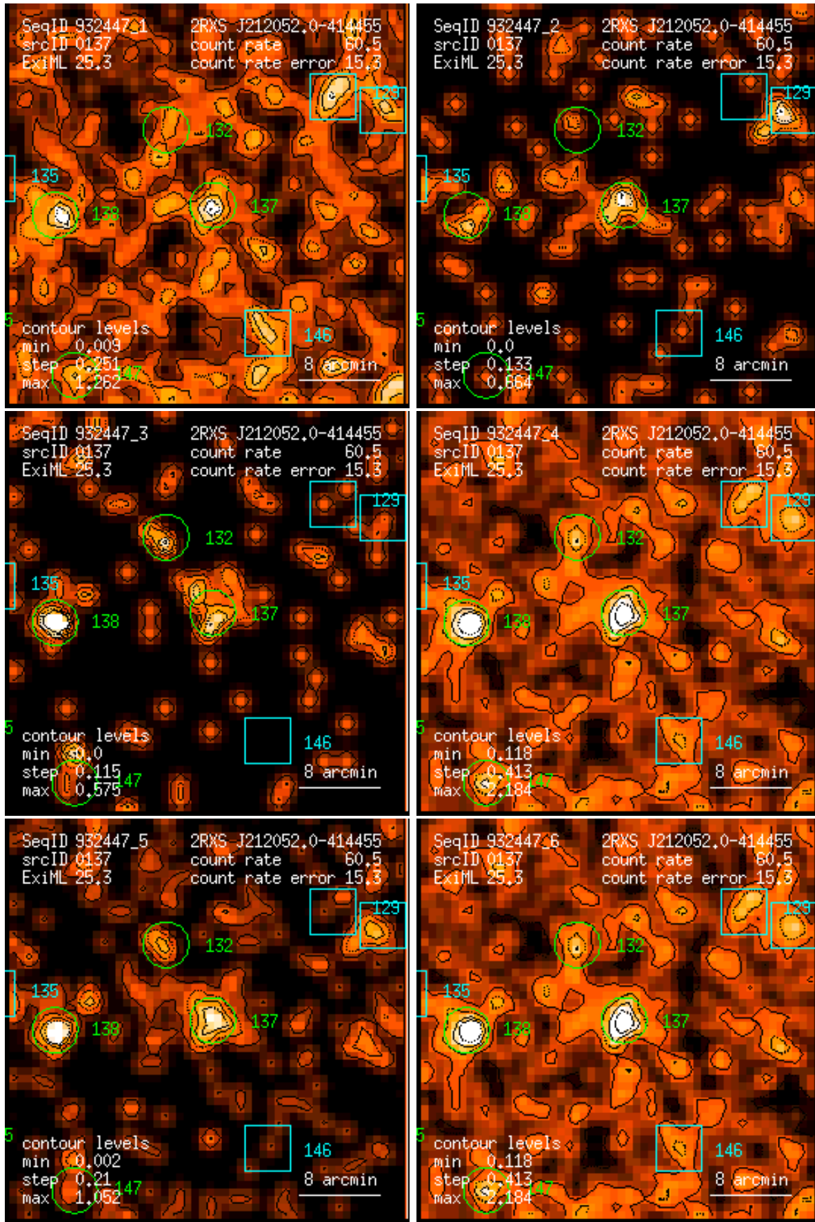
Figure 137: RASS 932447: detection 0137: band rate images, Gaussian filter: (1) PSPC channels 11 – 41, (2) 52 – 90, (3) 91 – 201, (4) 11 – 235, (5) 52 – 201, (6) 11 – 201. Broad band rates in counts/ks. Band rate contour levels in counts/ks/arcmin 2 .
