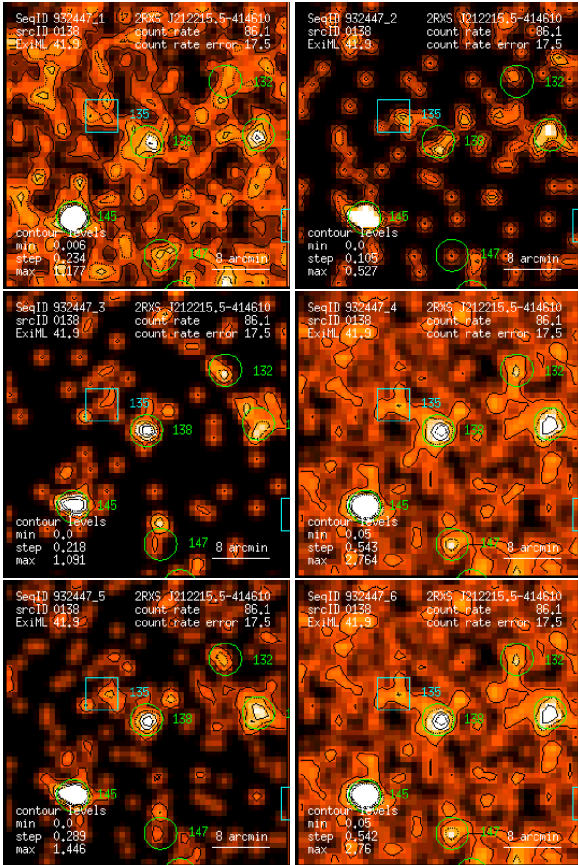
Figure 138: RASS 932447: detection 0138: band rate images, Gaussian filter: (1) PSPC channels 11 – 41, (2) 52 – 90, (3) 91 – 201, (4) 11 – 235, (5) 52 – 201, (6) 11 – 201. Broad band rates in counts/ks. Band rate contour levels in counts/ks/arcmin 2 .
