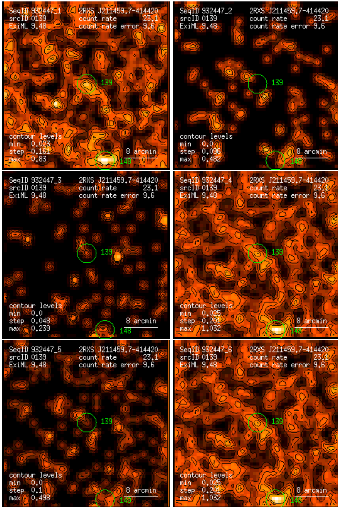
Figure 139: RASS 932447: detection 0139: band rate images, Gaussian filter: (1) PSPC channels 11 – 41, (2) 52 – 90, (3) 91 – 201, (4) 11 – 235, (5) 52 – 201, (6) 11 – 201. Broad band rates in counts/ks. Band rate contour levels in counts/ks/arcmin 2 .
