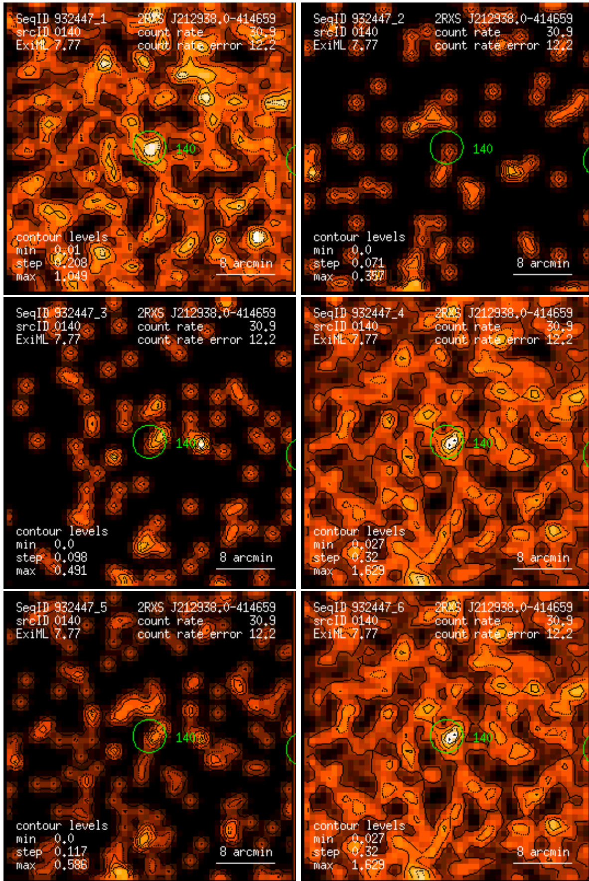
Figure 140: RASS 932447: detection 0140: band rate images, Gaussian filter: (1) PSPC channels 11 – 41, (2) 52 – 90, (3) 91 – 201, (4) 11 – 235, (5) 52 – 201, (6) 11 – 201. Broad band rates in counts/ks. Band rate contour levels in counts/ks/arcmin 2 .
