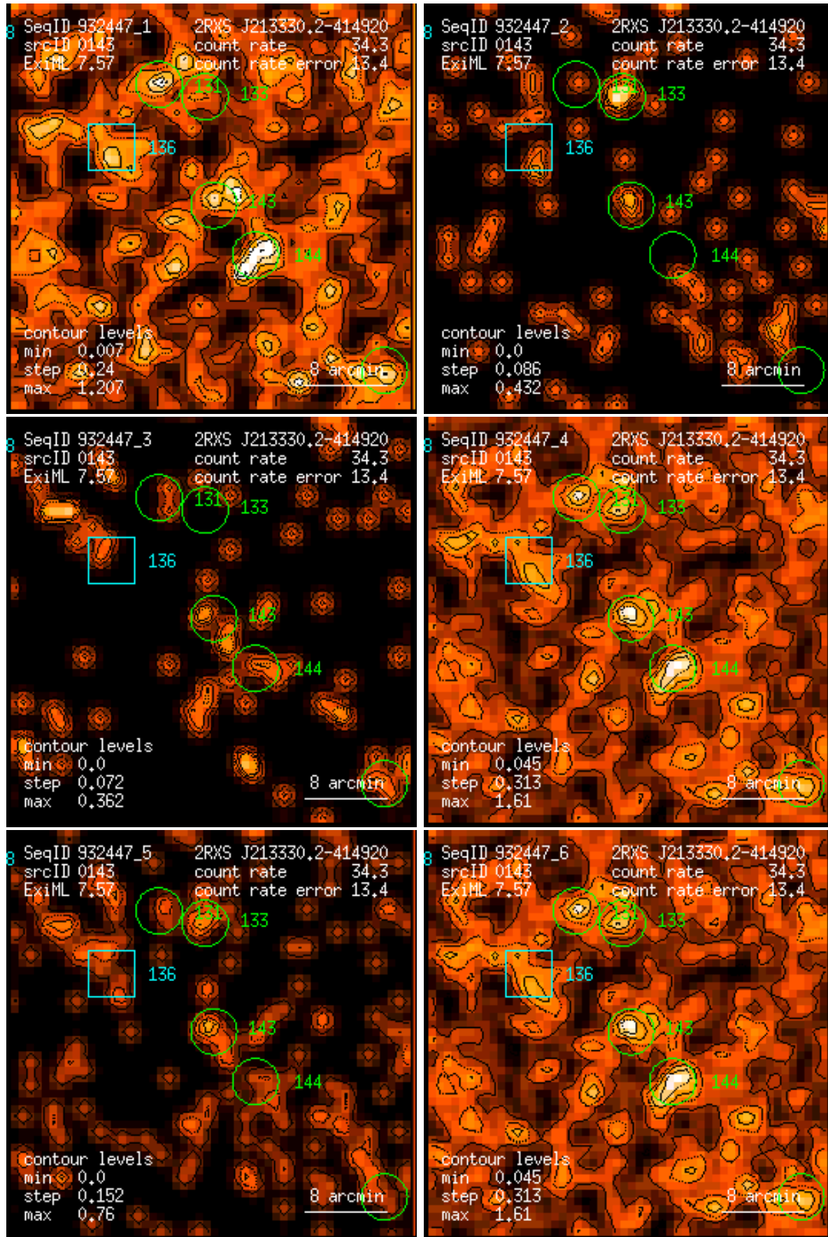
Figure 143: RASS 932447: detection 0143: band rate images, Gaussian filter: (1) PSPC channels 11 – 41, (2) 52 – 90, (3) 91 – 201, (4) 11 – 235, (5) 52 – 201, (6) 11 – 201. Broad band rates in counts/ks. Band rate contour levels in counts/ks/arcmin 2 .
