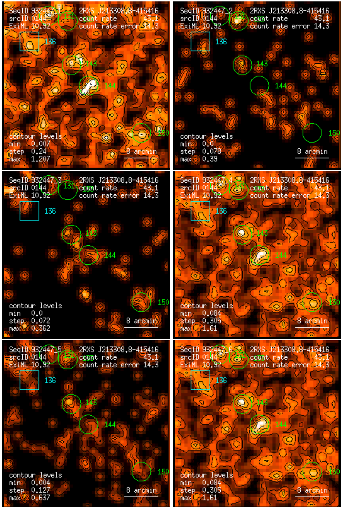
Figure 144: RASS 932447: detection 0144: band rate images, Gaussian filter: (1) PSPC channels 11 – 41, (2) 52 – 90, (3) 91 – 201, (4) 11 – 235, (5) 52 – 201, (6) 11 – 201. Broad band rates in counts/ks. Band rate contour levels in counts/ks/arcmin 2 .
