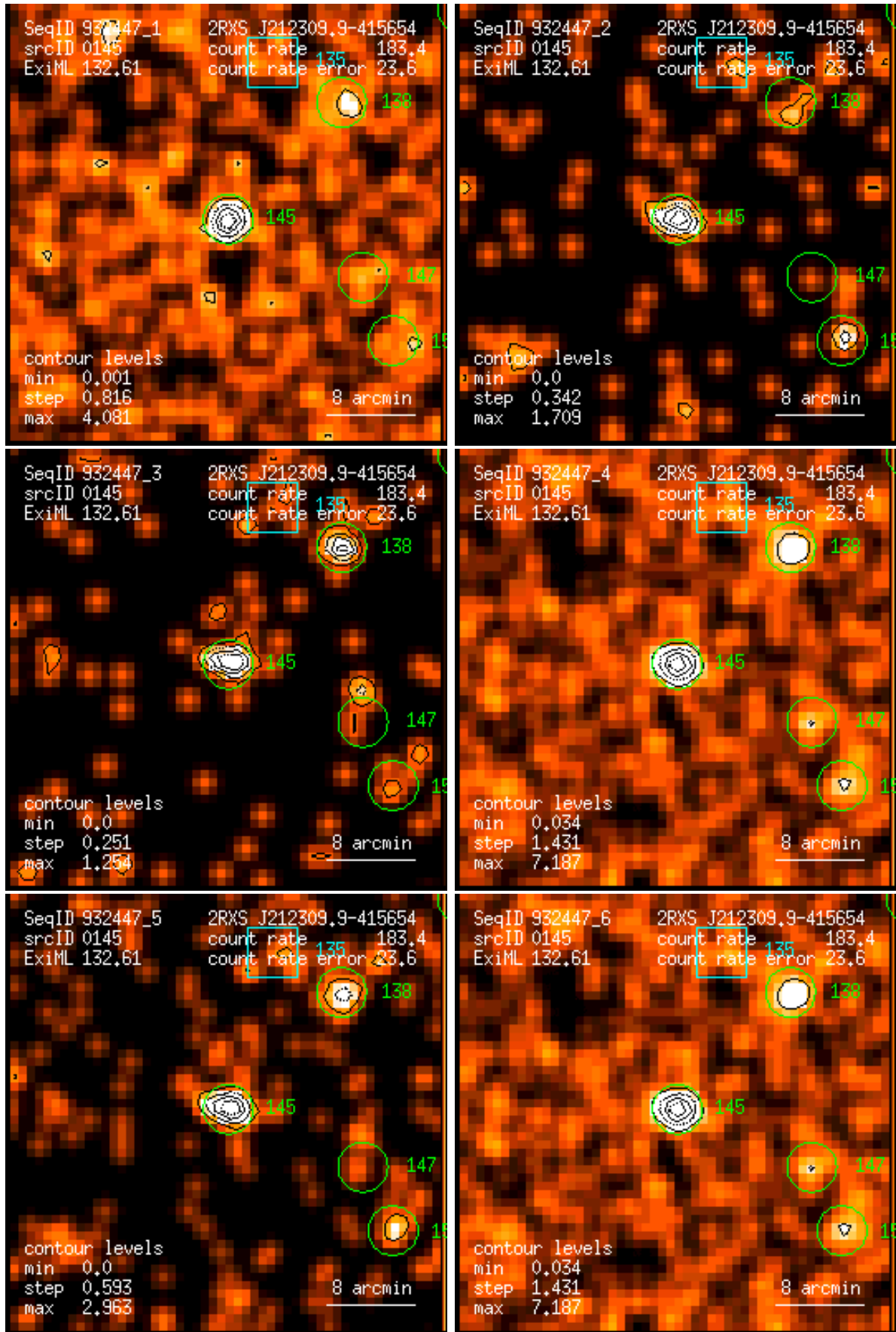
Figure 145: RASS 932447: detection 0145: band rate images, Gaussian filter: (1) PSPC channels 11 – 41, (2) 52 – 90, (3) 91 – 201, (4) 11 – 235, (5) 52 – 201, (6) 11 – 201. Broad band rates in counts/ks. Band rate contour levels in counts/ks/arcmin 2 .
