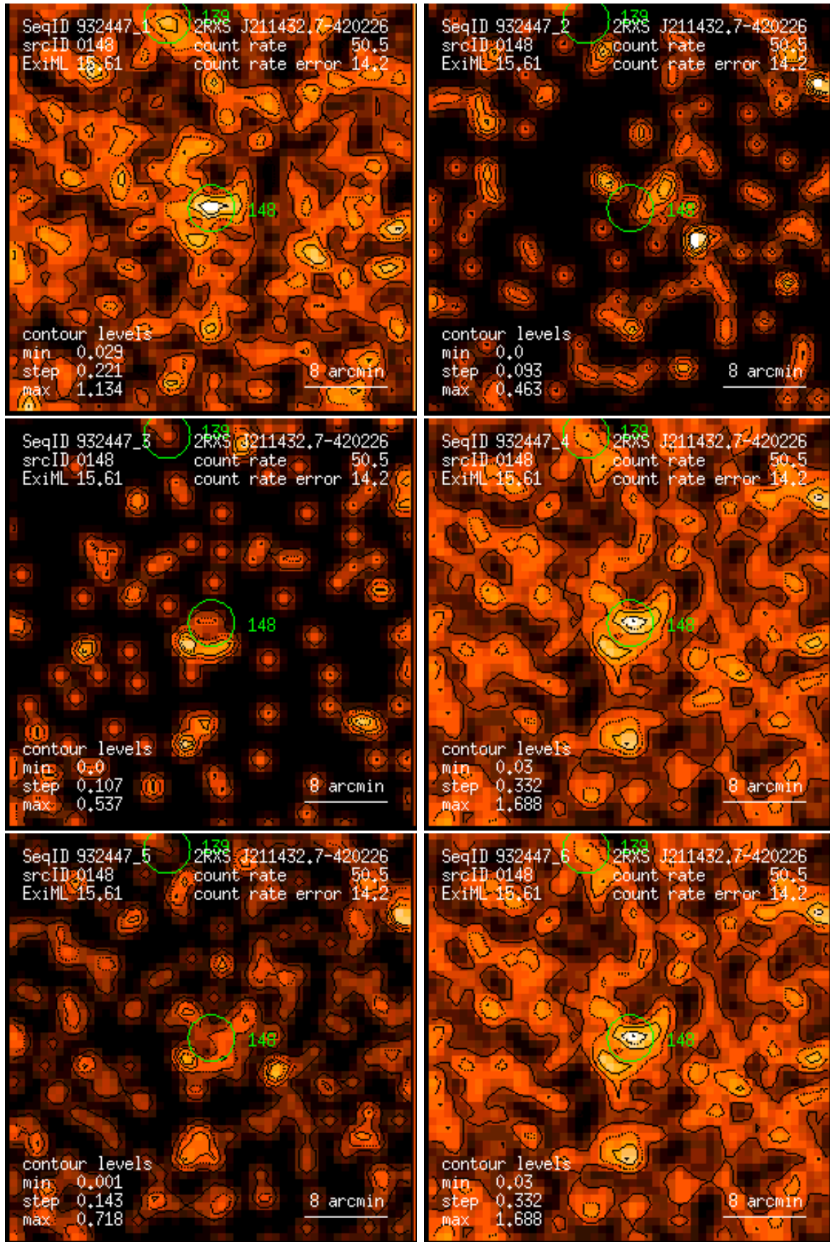
Figure 148: RASS 932447: detection 0148: band rate images, Gaussian filter: (1) PSPC channels 11 – 41, (2) 52 – 90, (3) 91 – 201, (4) 11 – 235, (5) 52 – 201, (6) 11 – 201. Broad band rates in counts/ks. Band rate contour levels in counts/ks/arcmin 2 .
