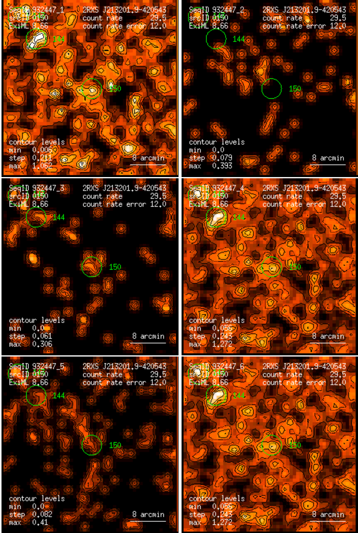
Figure 150: RASS 932447: detection 0150: band rate images, Gaussian filter: (1) PSPC channels 11 – 41, (2) 52 – 90, (3) 91 – 201, (4) 11 – 235, (5) 52 – 201, (6) 11 – 201. Broad band rates in counts/ks. Band rate contour levels in counts/ks/arcmin 2 .
