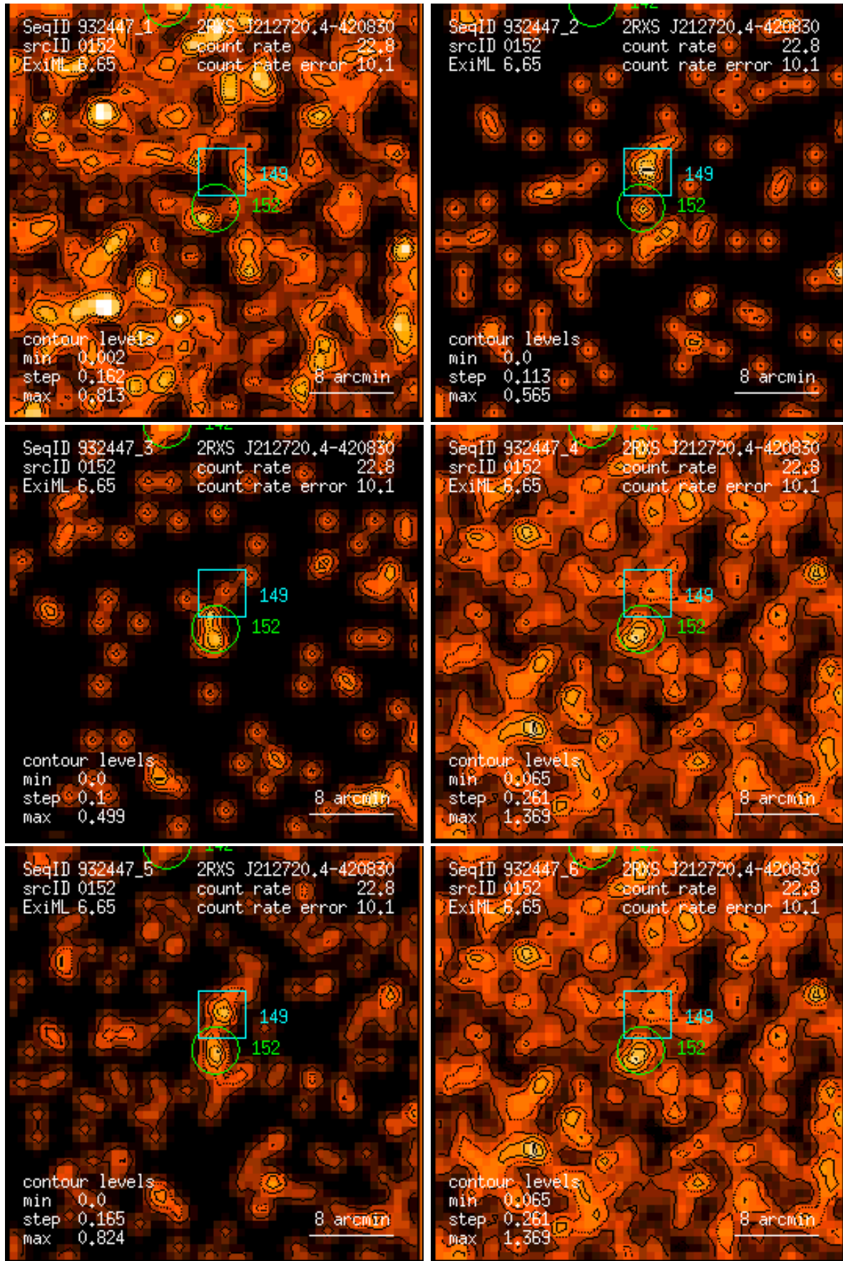
Figure 152: RASS 932447: detection 0152: band rate images, Gaussian filter: (1) PSPC channels 11 – 41, (2) 52 – 90, (3) 91 – 201, (4) 11 – 235, (5) 52 – 201, (6) 11 – 201. Broad band rates in counts/ks. Band rate contour levels in counts/ks/arcmin 2 .
