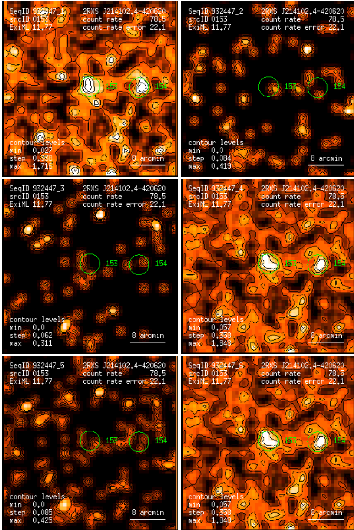
Figure 153: RASS 932447: detection 0153: band rate images, Gaussian filter: (1) PSPC channels 11 – 41, (2) 52 – 90, (3) 91 – 201, (4) 11 – 235, (5) 52 – 201, (6) 11 – 201. Broad band rates in counts/ks. Band rate contour levels in counts/ks/arcmin 2 .
