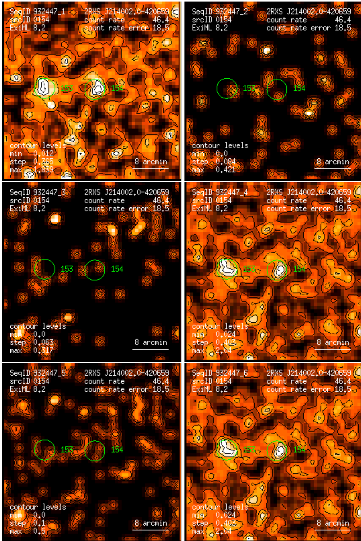
Figure 154: RASS 932447: detection 0154: band rate images, Gaussian filter: (1) PSPC channels 11 – 41, (2) 52 – 90, (3) 91 – 201, (4) 11 – 235, (5) 52 – 201, (6) 11 – 201. Broad band rates in counts/ks. Band rate contour levels in counts/ks/arcmin 2 .
