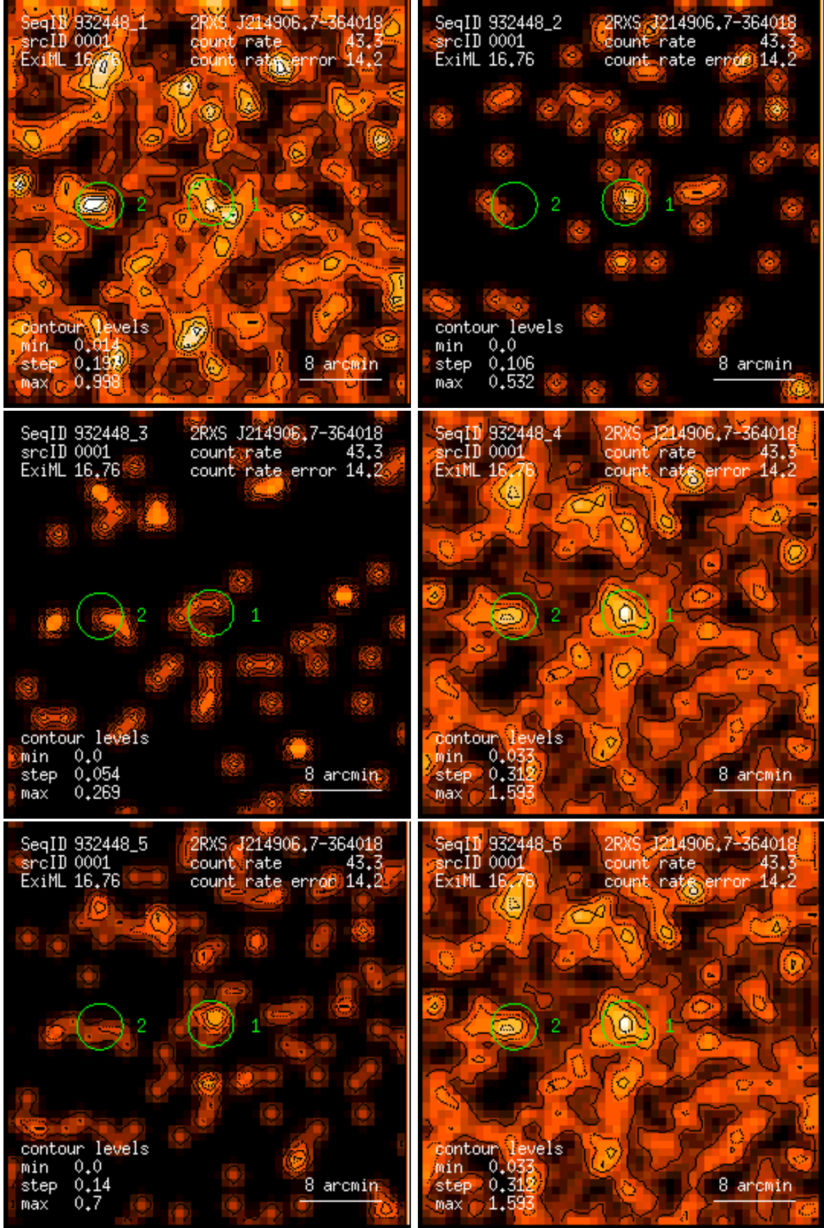
Figure 1: RASS 932448: detection 0001: band rate images, Gaussian filter: (1) PSPC channels 11 – 41, (2) 52 – 90, (3) 91 – 201, (4) 11 – 235, (5) 52 – 201, (6) 11 – 201. Broad band rates in counts/ks. Band rate contour levels in counts/ks/arcmin 2 .
