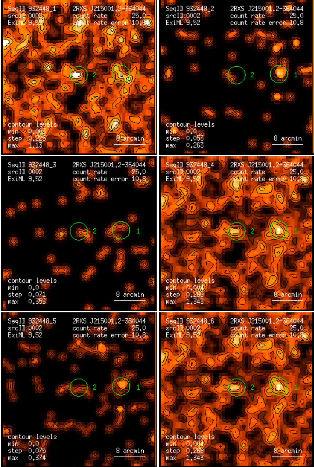
Figure 2: RASS 932448: detection 0002: band rate images, Gaussian filter: (1) PSPC channels 11 – 41, (2) 52 – 90, (3) 91 – 201, (4) 11 – 235, (5) 52 – 201, (6) 11 – 201. Broad band rates in counts/ks. Band rate contour levels in counts/ks/arcmin 2 .
